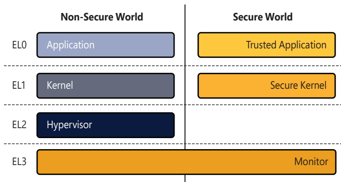
FIGURE 9-22 The ARM64 execution environment.
