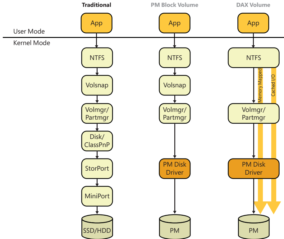
FIGURE 11-76 Device I/O stack comparison between traditional volumes, block mode volumes, and DAX volumes.
