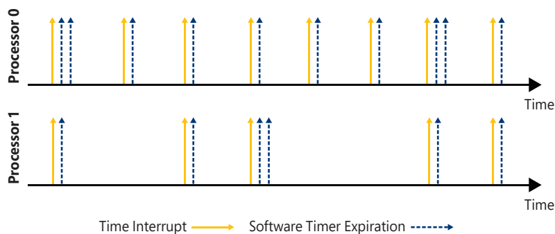
FIGURE 8-22 Intelligent timer tick distribution applied to processor 1.
