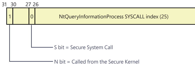
FIGURE 9-35 The Syscall selector number of the Secure Kernel.
