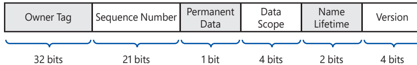
FIGURE 8-41 Format of a WNF state name.
