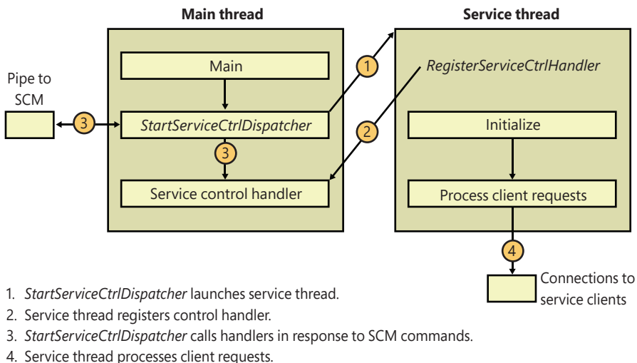
FIGURE 10-8 Inside a service process.
