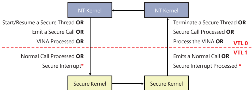
FIGURE 9-33 The VSM dispatch loop.
