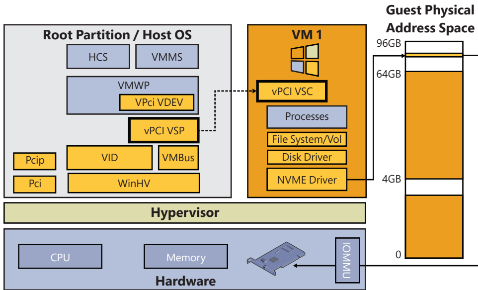
FIGURE 9-29 Hardware-accelerated devices.
