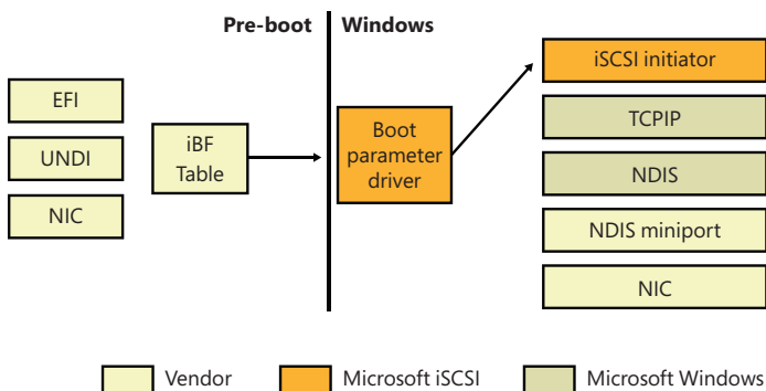
FIGURE 12-9 iSCSI boot architecture.
