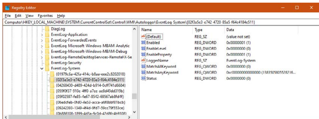
FIGURE 10-36 The EventLog-System Autologger’s enabled providers.
