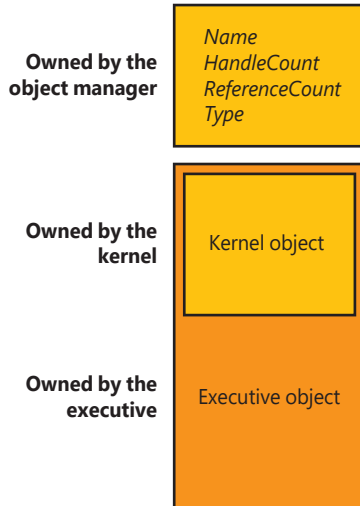
FIGURE 8-30 Executive objects that contain kernel objects.
