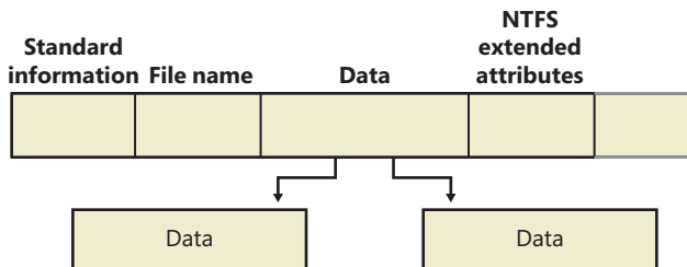
FIGURE 11-39 MFT file record for a large file with two data runs.
