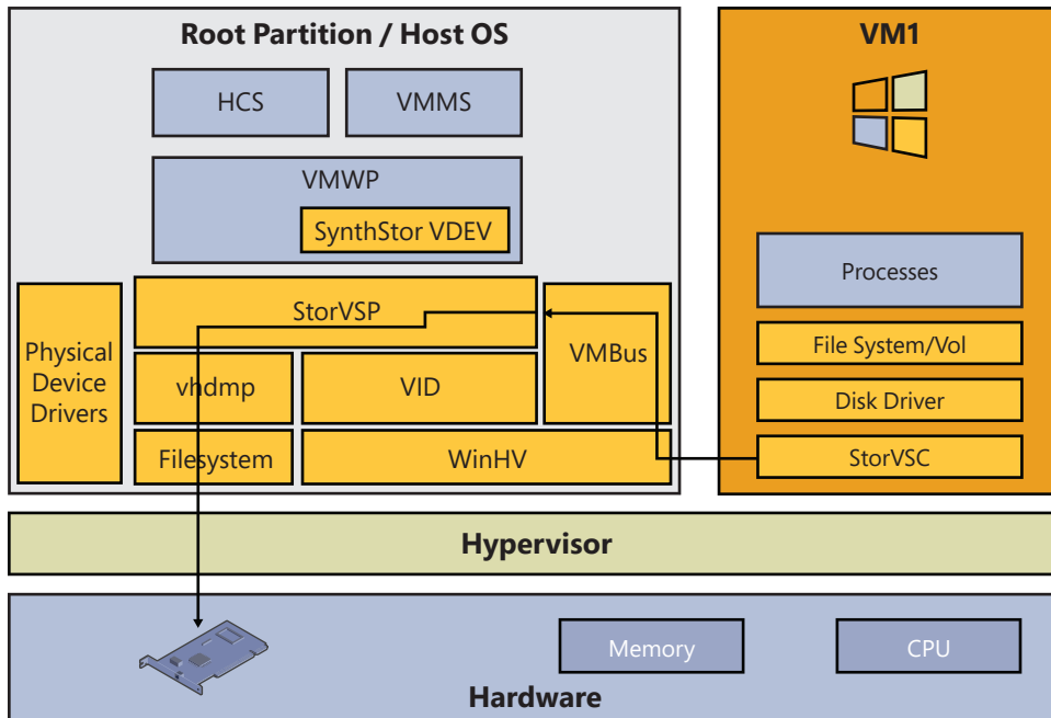
FIGURE 9-28 The storage controller paravirtualized device.
