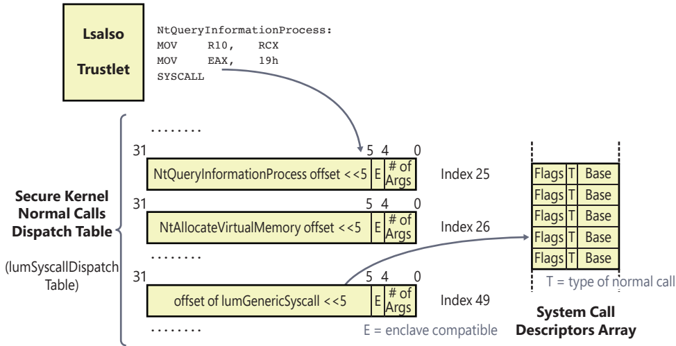
FIGURE 9-34 A trustlet performing a special normal call to the NtQueryInformationProcess API.
