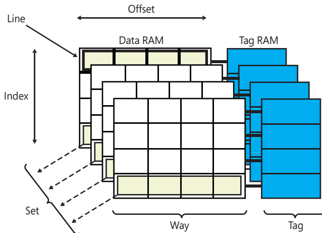
FIGURE 8-5 A four-way set associative cache.
