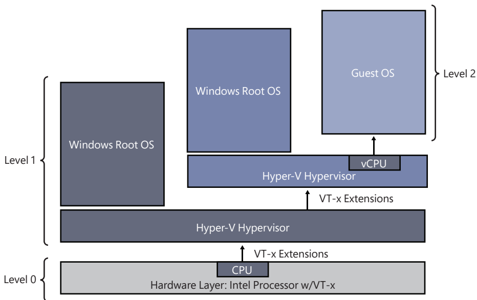
FIGURE 9-20 Nested virtualization scheme.
