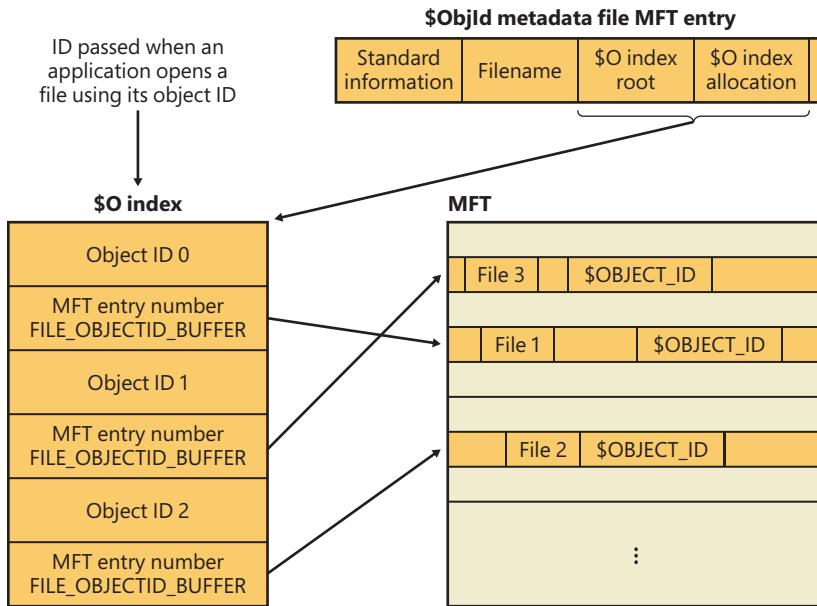
FIGURE 11-51 $ObjId and $OBJECT_ID relationships.
