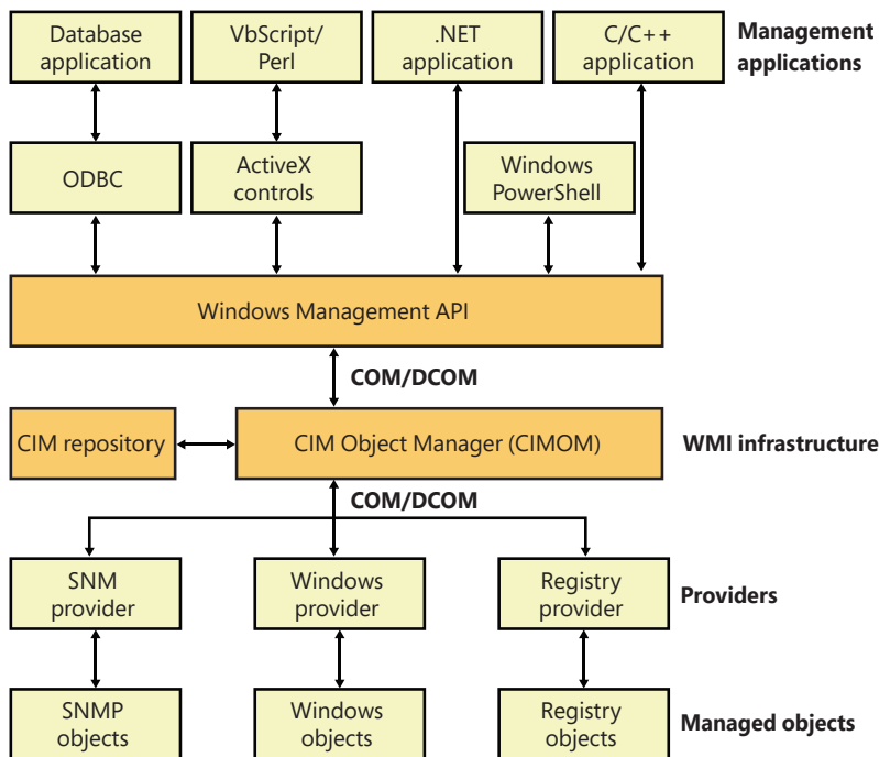
FIGURE 10-27 WMI architecture.
