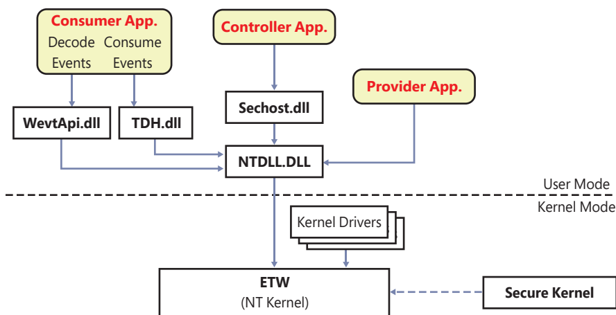
FIGURE 10-31 ETW architecture.
