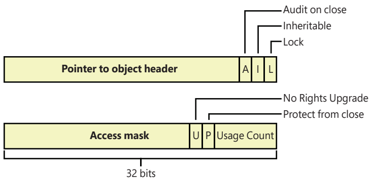
FIGURE 8-34 Structure of a 32-bit handle table entry.
