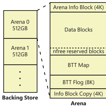
FIGURE 11-75 Layout of a DAX disk that supports sector atomicity (BTT algorithm).
