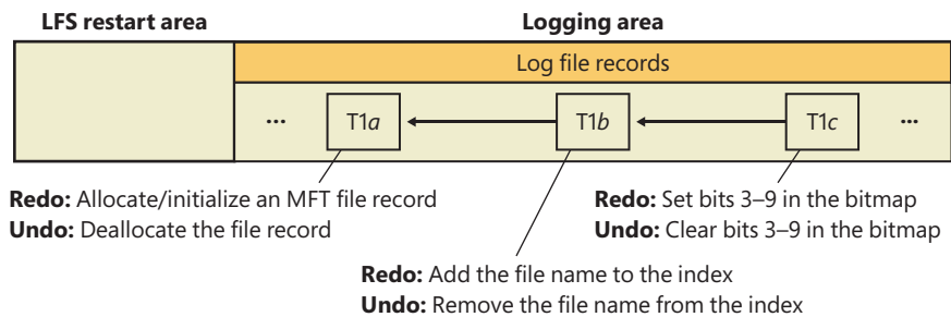
FIGURE 11-58 Update records in the log file.
