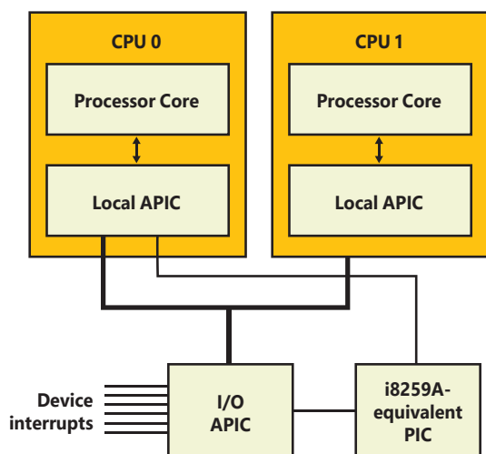
FIGURE 8-12 APIC architecture.
