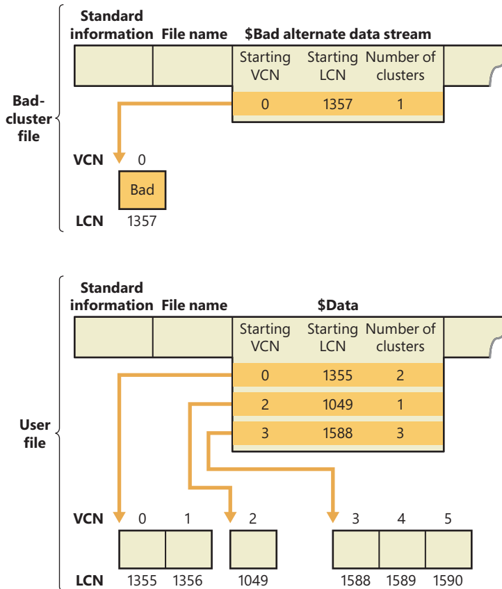
FIGURE 11-65 Bad-cluster remapping.
