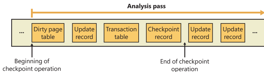
FIGURE 11-60 Analysis pass.
