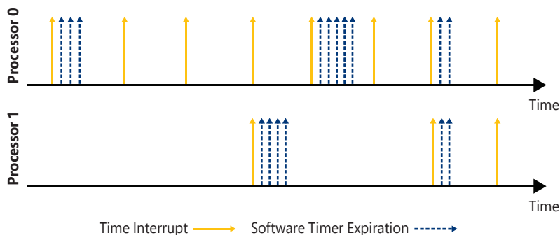
FIGURE 8-23 Timer coalescing.
