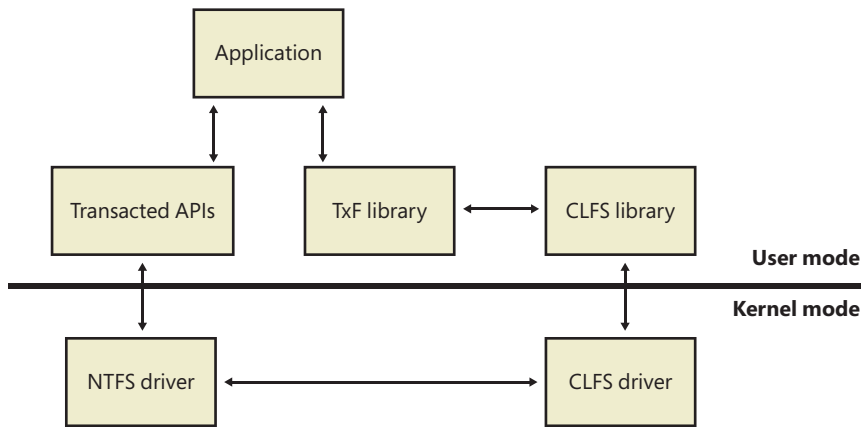
FIGURE 11-54 TxF architecture.
