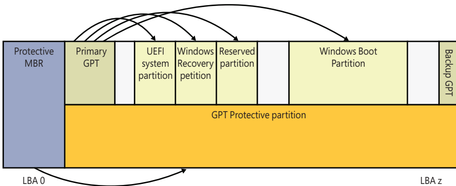
FIGURE 12-2 Sample UEFI hard disk layout.
