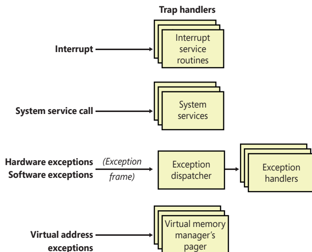
FIGURE 8-11 Trap dispatching.
