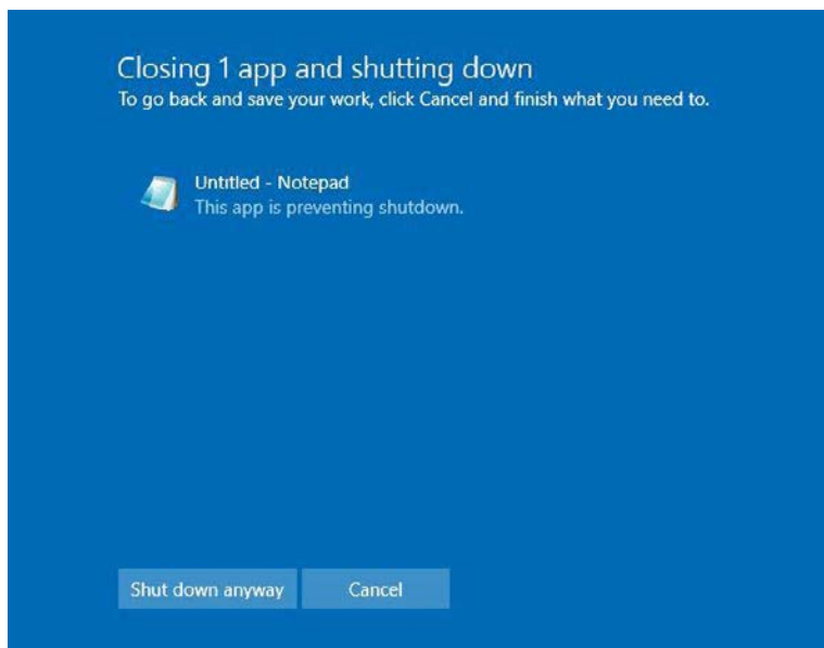
FIGURE 12-14 Hung-program screen.
