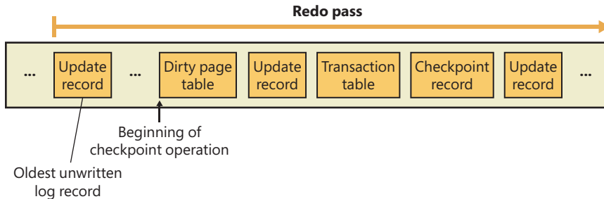
FIGURE 11-61 Redo pass.
