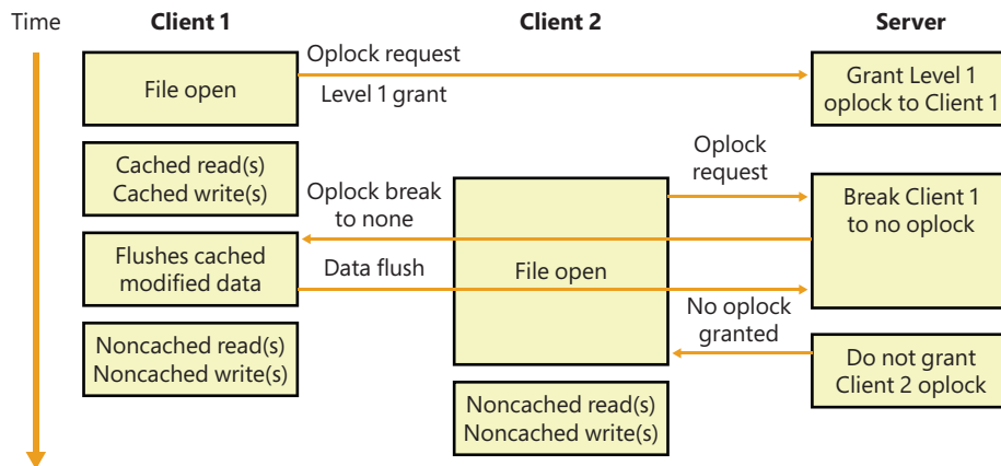
FIGURE 11-19 Oplock example.
