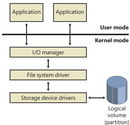
FIGURE 11-17 Local FSD.
