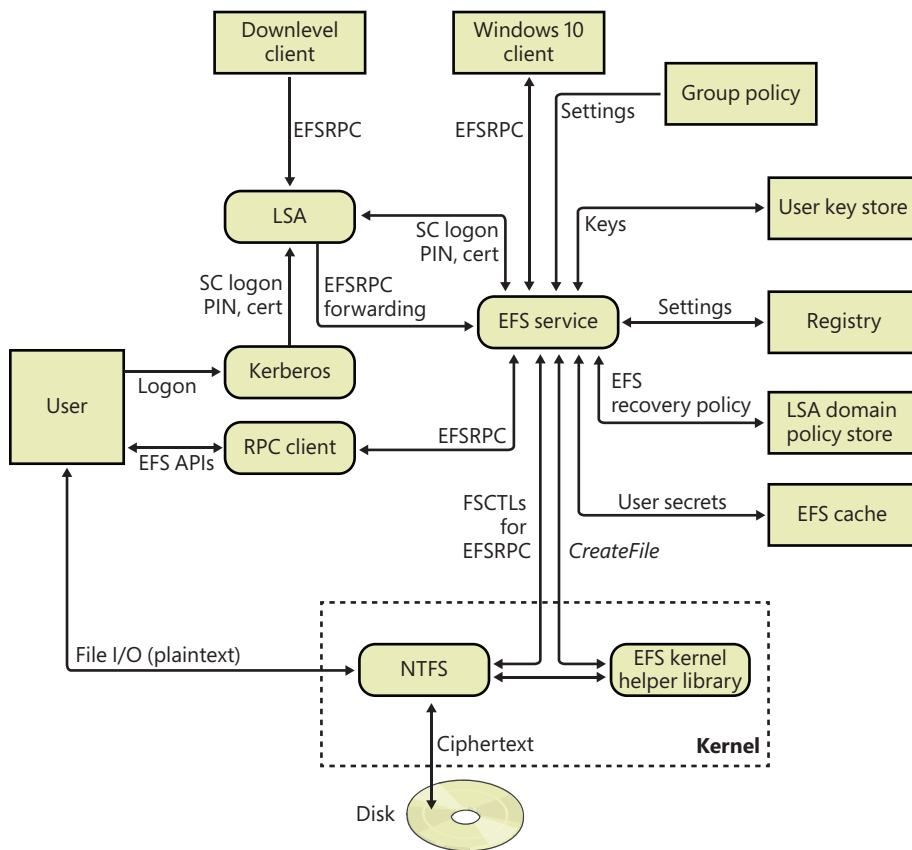
FIGURE 11-69 EFS architecture.
