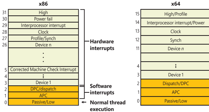
FIGURE 8-13 x86 and x64 interrupt request levels (IRQLs).
