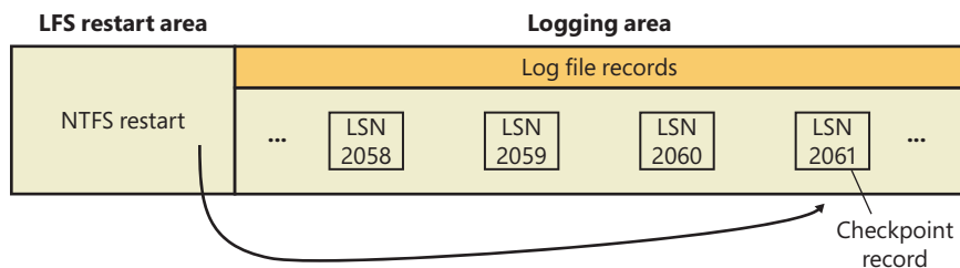
FIGURE 11-59 Checkpoint record in the log file.
