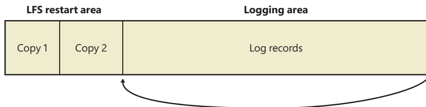
FIGURE 11-57 Log file regions.
