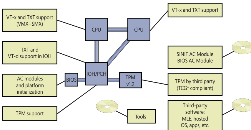
FIGURE 12-7 Intel TXT (Trusted Execution Technology) components.
