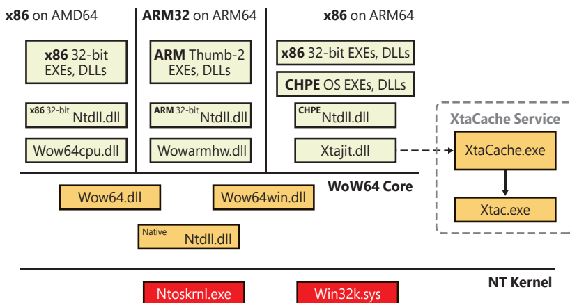
FIGURE 8-28 The WoW64 architecture.
