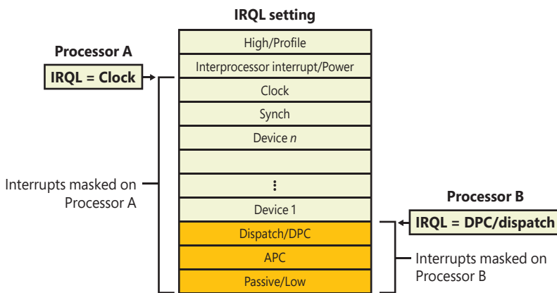
FIGURE 8-14 Masking interrupts.
