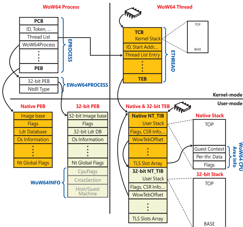
FIGURE 8-29 Internal configuration of a WoW64 process with only a single thread.
