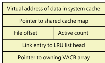
FIGURE 11-7 VACB data structure.
