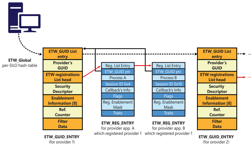
FIGURE 10-34 The ETW_GUID_ENTRY data structure and the ETW_REG_ENTRY .
