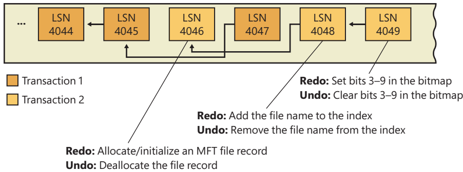
FIGURE 11-63 Undoing a transaction.
