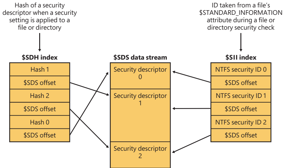
FIGURE 11-53 $Secure indexing.
