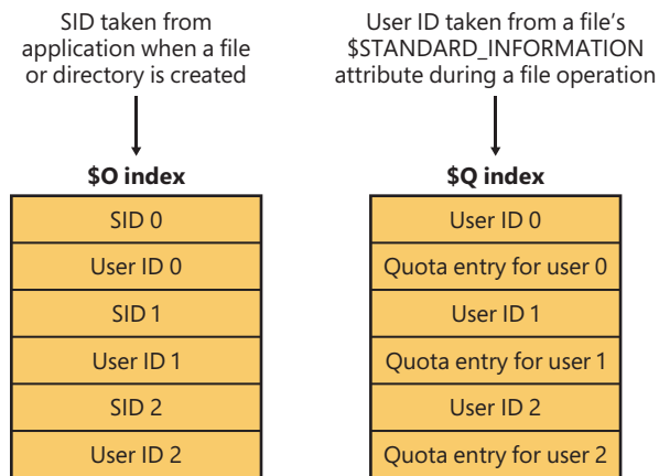
FIGURE 11-52 $Quota indexing.
