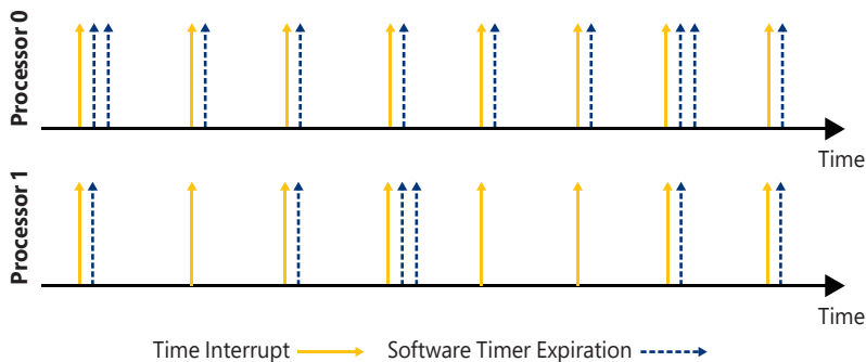
FIGURE 8-20 Timer expiration.
