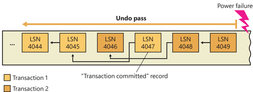
FIGURE 11-62 Undo pass.
