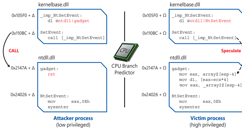
FIGURE 8-7 A scheme of Spectre attack Variant 2.
