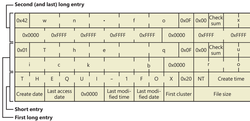
FIGURE 11.16 FAT directory entry.
