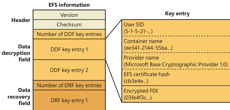
FIGURE 11-70 Format of EFS information and key entries.
