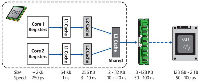
FIGURE 8-2 Caches and storage memory of modern CPUs and their average size and access time.
