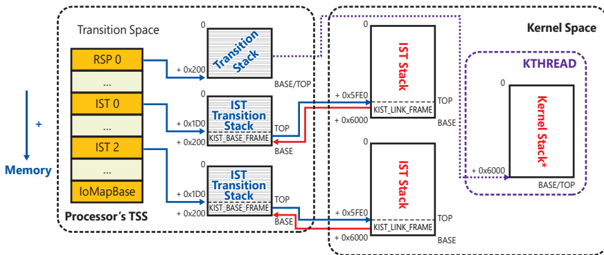
FIGURE 8-8 Configuration of the CPU's Task State Segment (TSS) when KVA shadowing is active.
