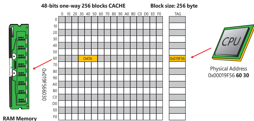
FIGURE 8-4 A sample 48-bit one-way CPU cache.
