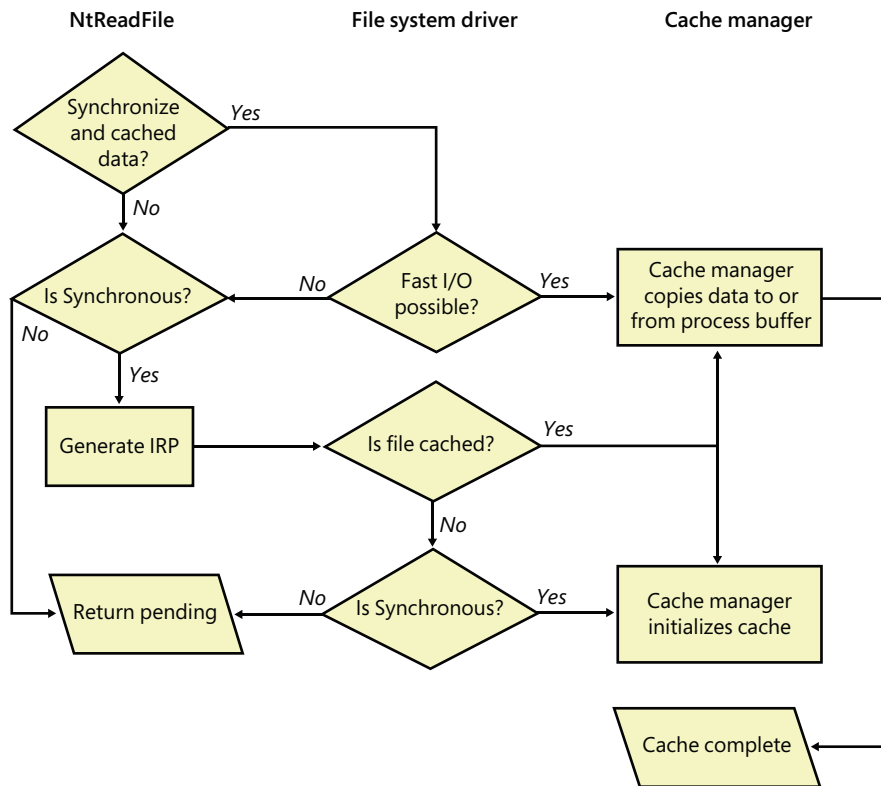
FIGURE 11-12 Fast I/O decision tree.
