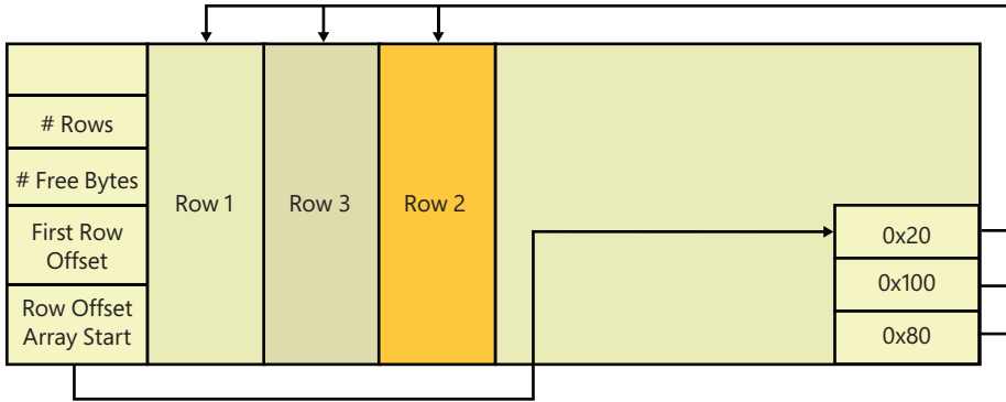
FIGURE 11-80 A leaf bucket with three index entries that are ordered by the array of offsets in the footer.
