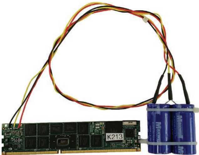
FIGURE 11-73 An NVDIMM, which has DRAM and Flash chips. An attached battery or on-board supercapacitors are needed for maintaining the data in the DRAM chips.
