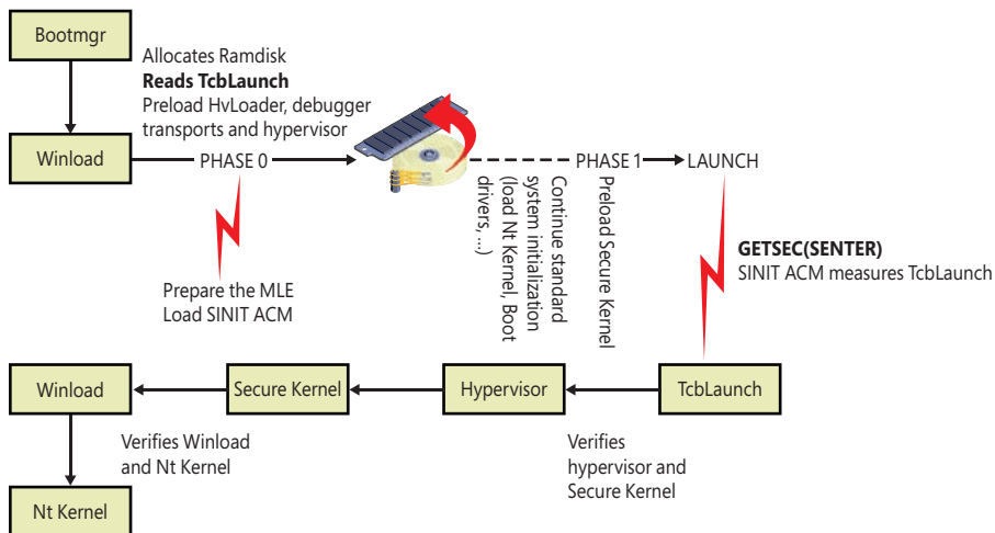
FIGURE 12-10 The Secure Launch scheme. Note that the hypervisor and Secure Kernel start from the RAM disk.
