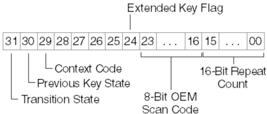
Figure 6–1. The six keystroke–message fields of the IParam variable.
