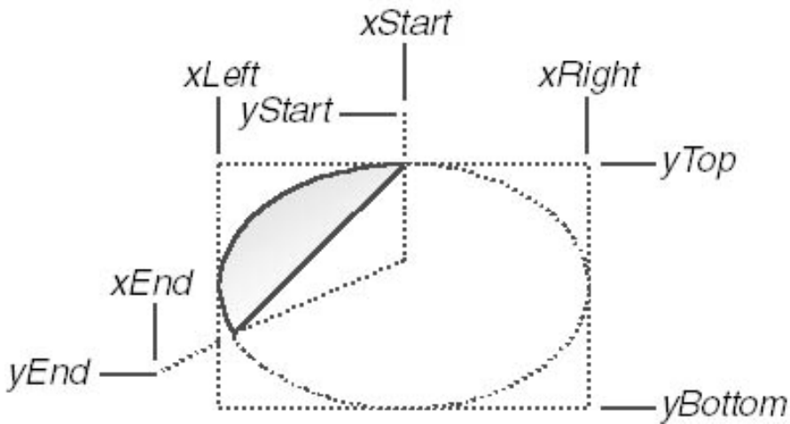
Figure 5–12. A figure drawn using the Chord function.
