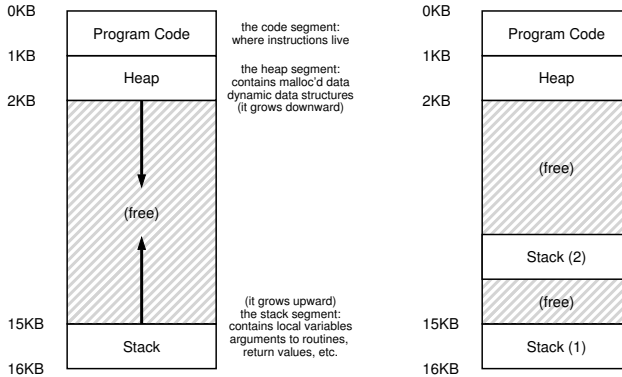
Figure 26.1: A Single-Threaded Address Space
