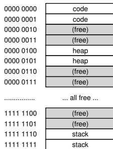
Figure 20.3: A 16-KB Address Space With 64-byte Pages
