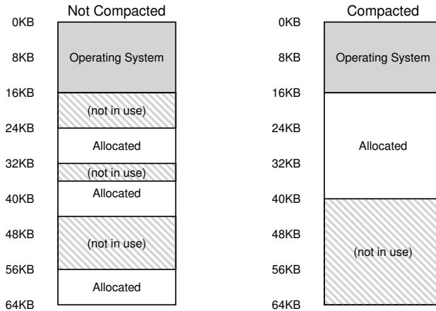
Figure 16.3: Non-compacted and Compacted Memory
