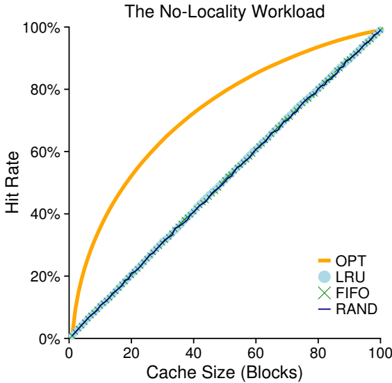
Figure 22.2: The No-Locality Workload
