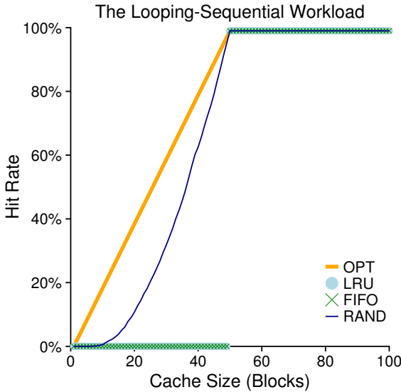
Figure 22.4: The Looping Workload
