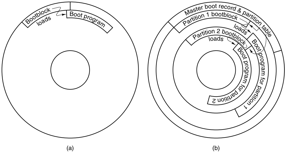
Figure 2-36. Disk structures used for bootstrapping. (a) Unpartitioned disk. The first sector is the bootblock. (b) Partitioned disk. The first sector is the master boot record, also called masterboot .
