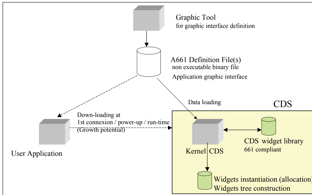
Figure 4.2.2 – Definition File Integration Process
