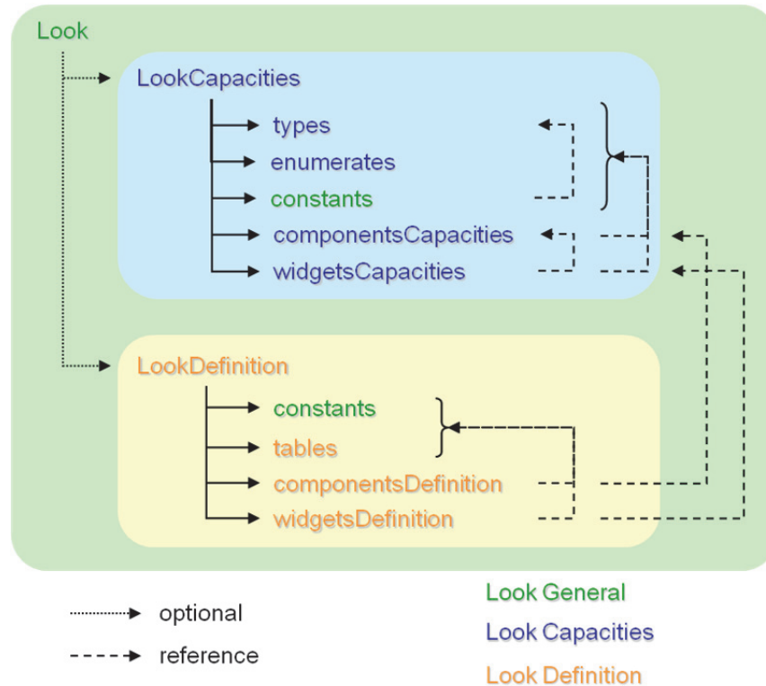
Figure J-4.1-1 – Look Modeling XML elements
