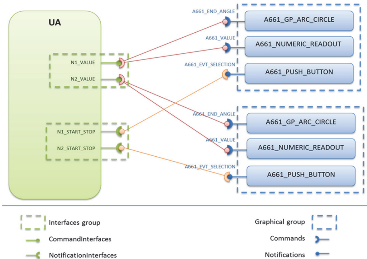
Figure K-2-1 Links CommandInterface-Command and NotificationInterface-Notification K-2.1 UA CDS Interface Capacities/UA CDS Interface Definition
