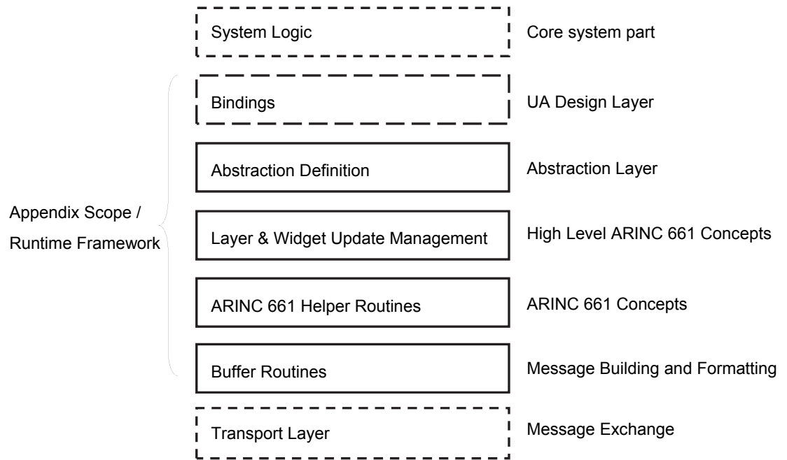
Figure I-4.4.2-1 – Full Abstraction (with Framework)
