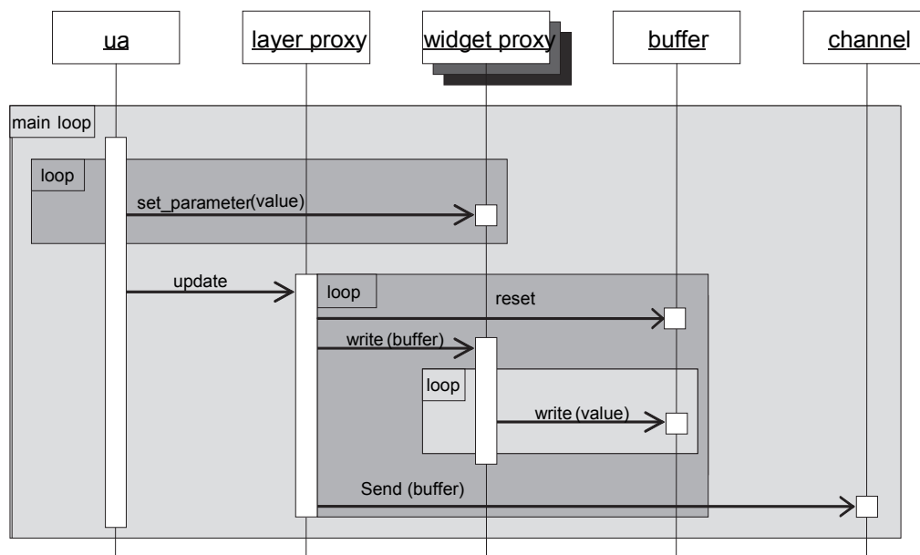
Figure I-4.3.2-1 – UA Production of ARINC 661 Objects
