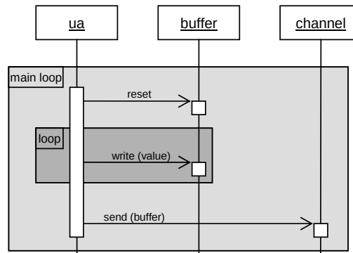
Figure I-3.1-1 – UA Production of ARINC 661 Buffers
