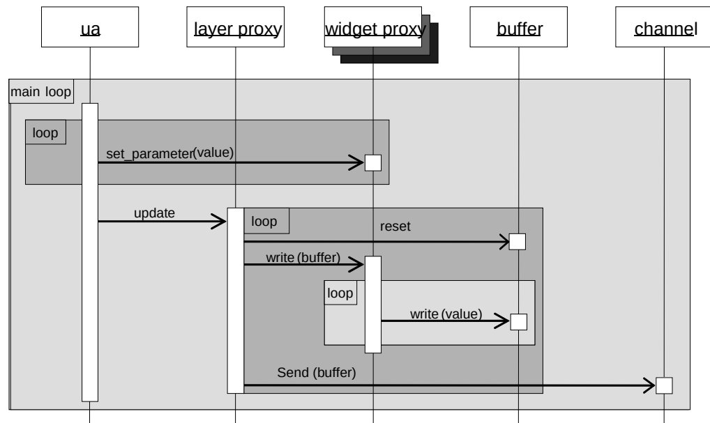
Figure I-3.1-1 – UA Production of ARINC 661 Objects
