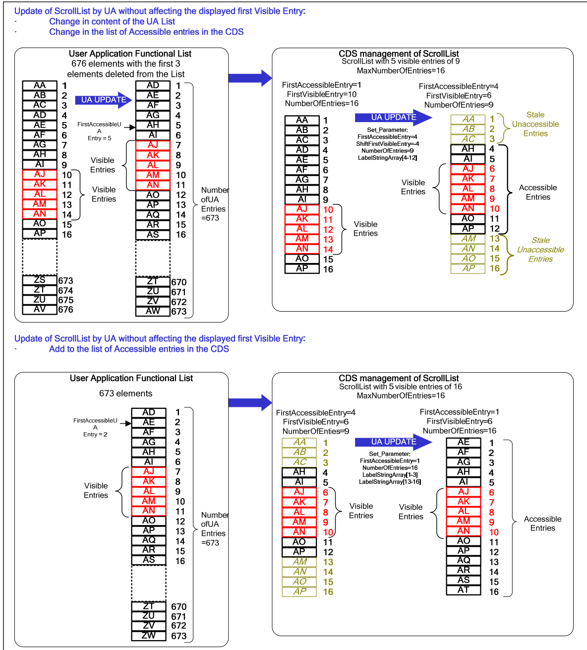
Figure 3.3.37-2 – Scroll List update using ShiftFirstVisibleEntry and FirstAccessibleEntry
