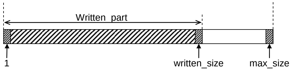
Figure I-4.1.1-1 – Writing to ARINC 661 Buffers
