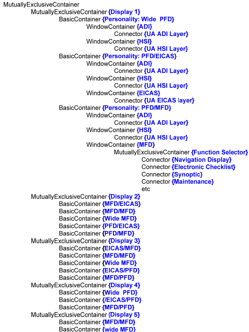
Figure H-3 - Super Layer Example
