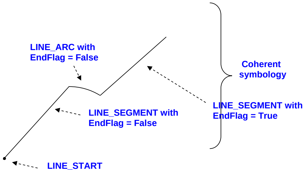
Figure E-2.4-2 – Example of a Line Item Group
