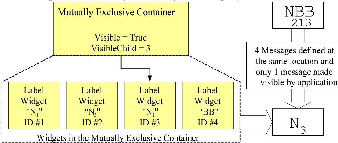
Figure 3.5.1-1 – Mutually Exclusive Container
