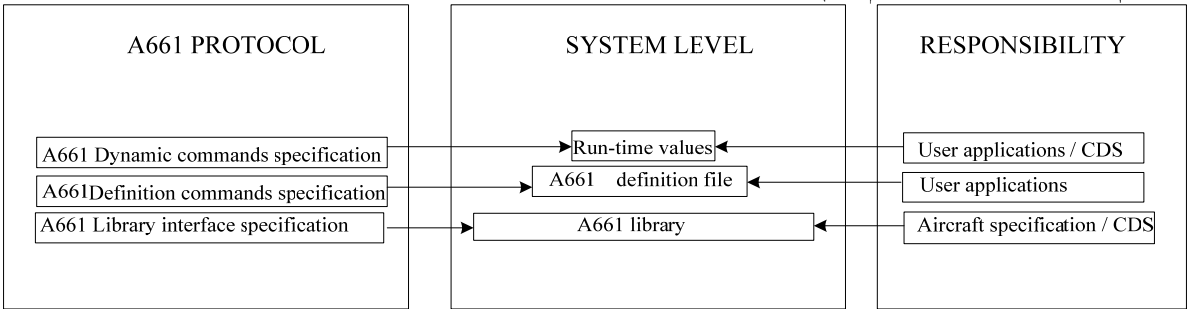
Figure 2.1-1 – ARINC 661 Protocol Principles
