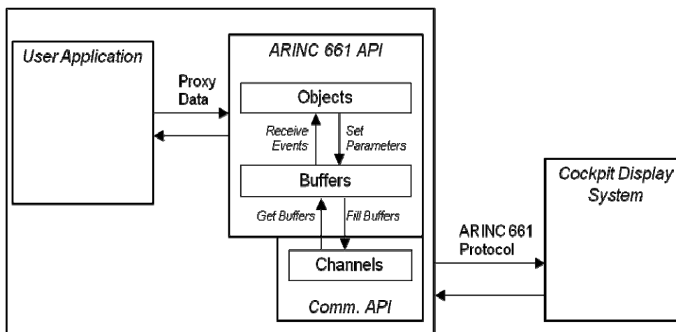
Figure I-2-2 – Example of ARINC 661 API Organization
