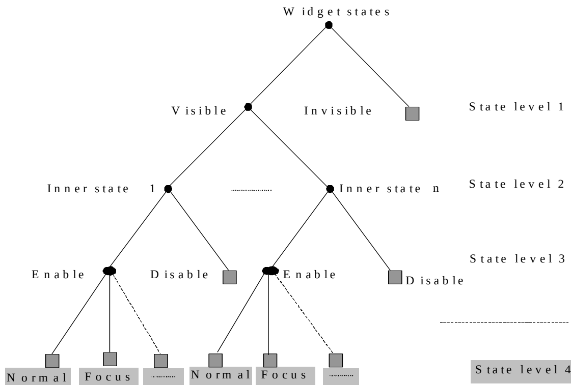
Figure 3.1.2.1 – Example of Widget States Levels
