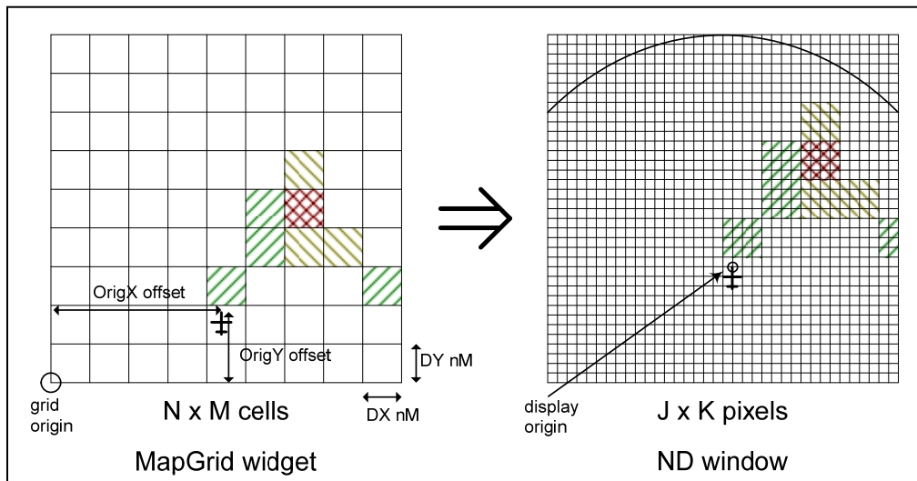
Figure 3.4.1 – Example MapGrid rendering in ND window
