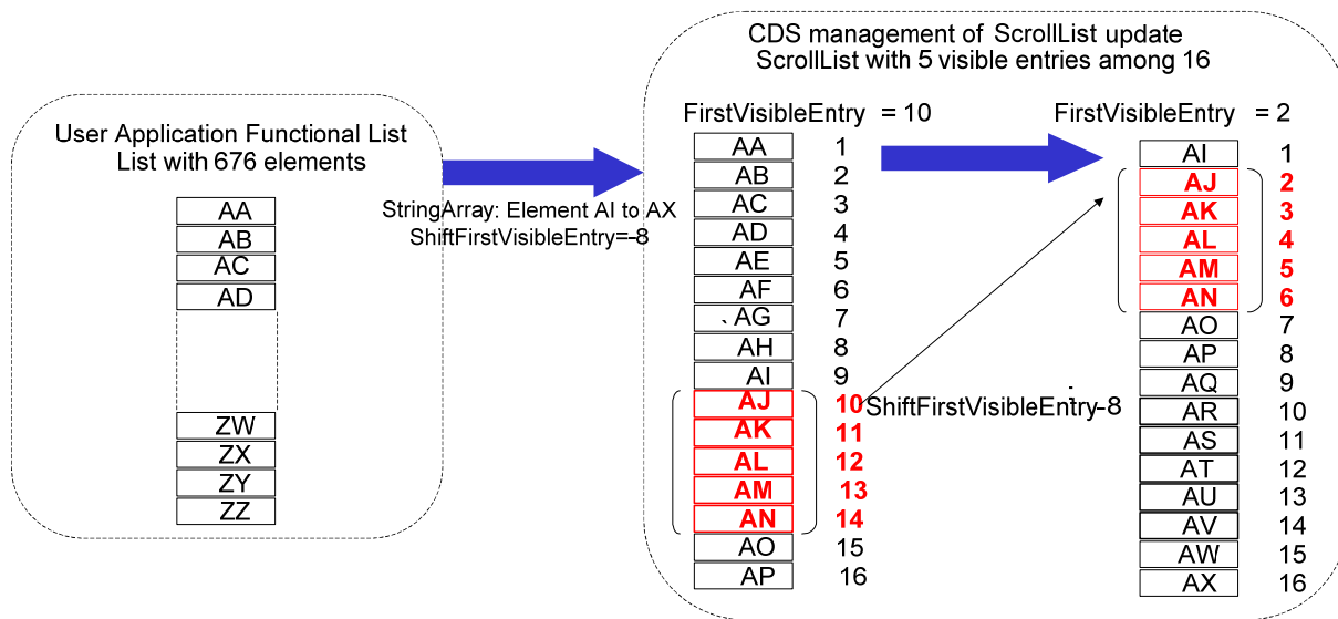
Figure 3.3.37-1 – Scroll List update using ShiftFirstVisibleEntry and LabelStringArray
