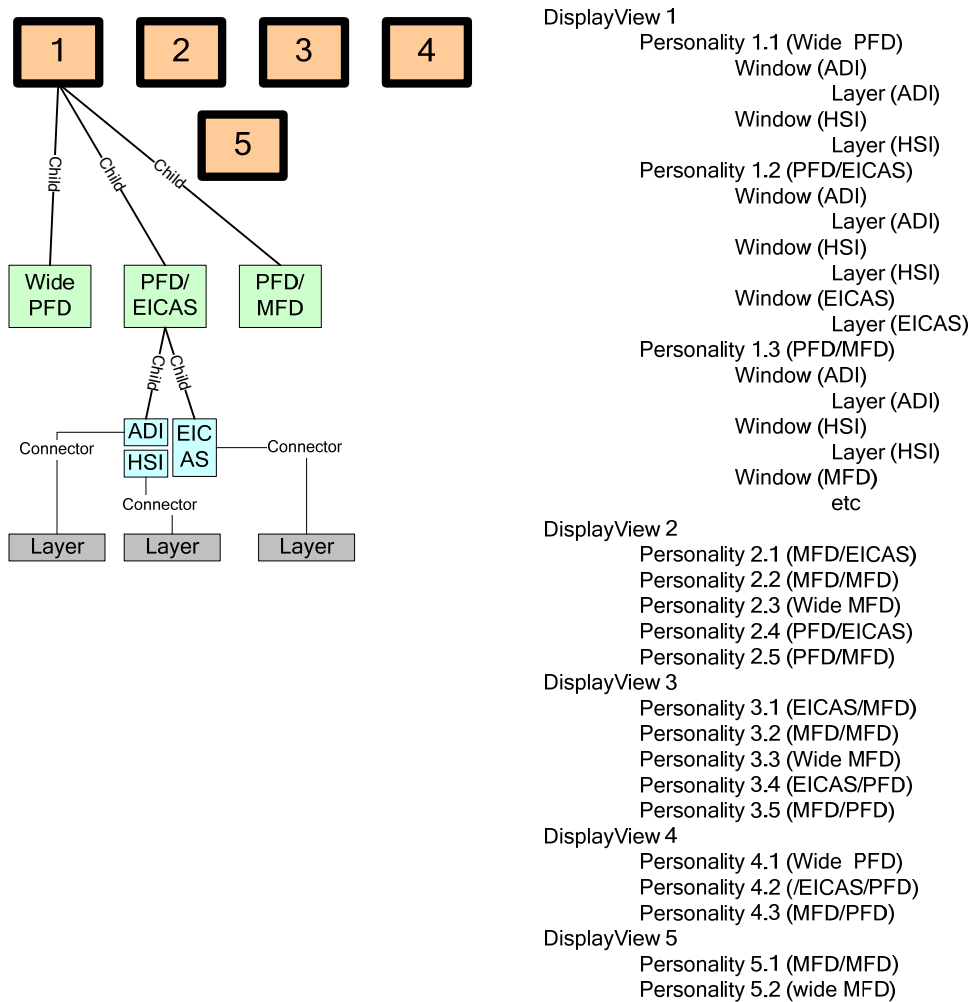
Figure H-2.2 – Example Schema Hierarchy
