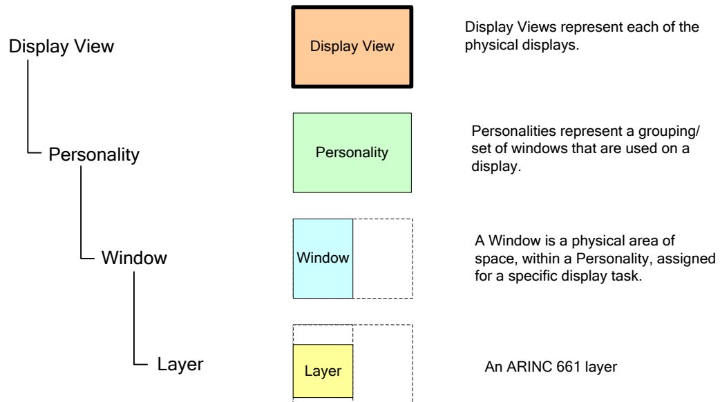
Figure H-2.1 – Display Surface Hierarchy
