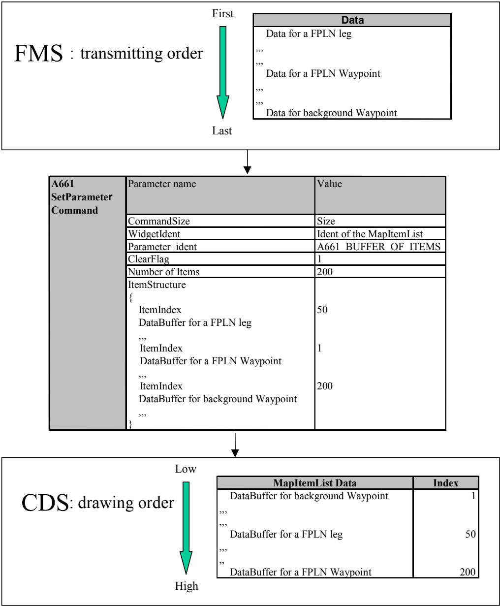
Figure E.4-1 - Example of Dynamic Priority Management
