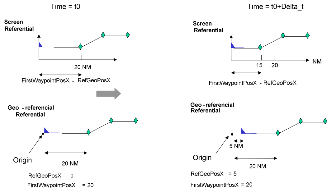
Figure 3.4.4-1 - Illustration of MapDataFormatX = A661_MDF_ABSOLUTE, X OriginOrigin is an Absolute Point
