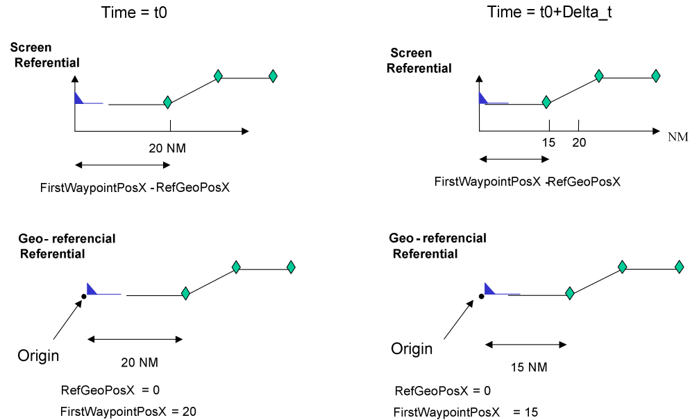
Figure 3.4.4-1 - Illustration of MapDataFormatX = A661_MDF_ABSOLUTE, X OriginOrigin is an Absolute Point
