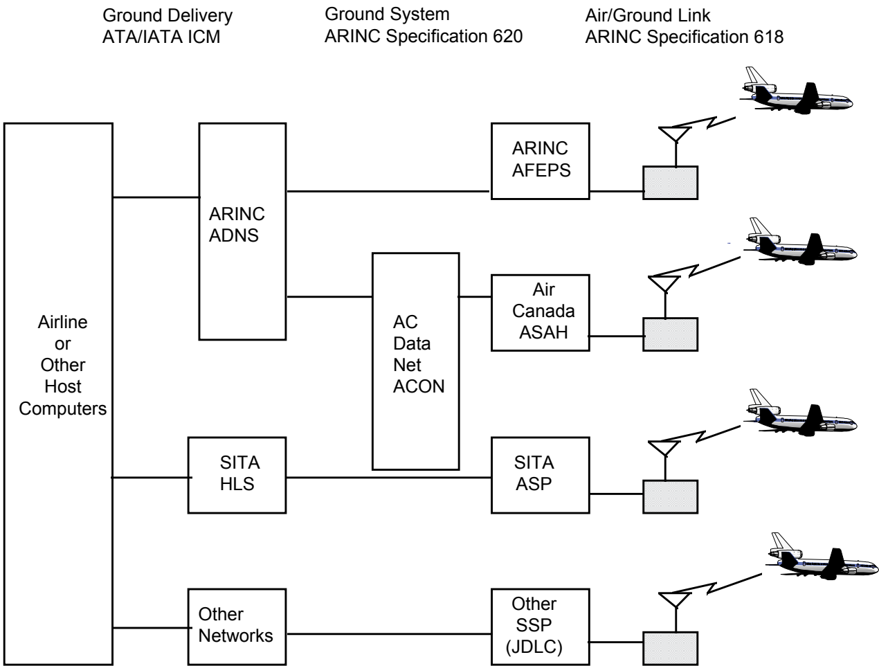
Figure 1-1 – Functional Depiction of Internetworking
