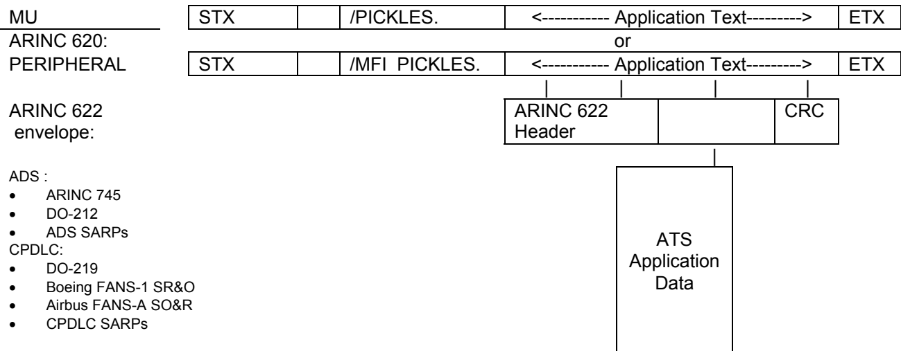
Figure 4.5-1 – ATS Message Encapsulation
