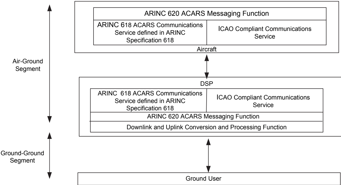
Figure 3.1.2-2 – ACARS Uplink/Downlink Architecture
