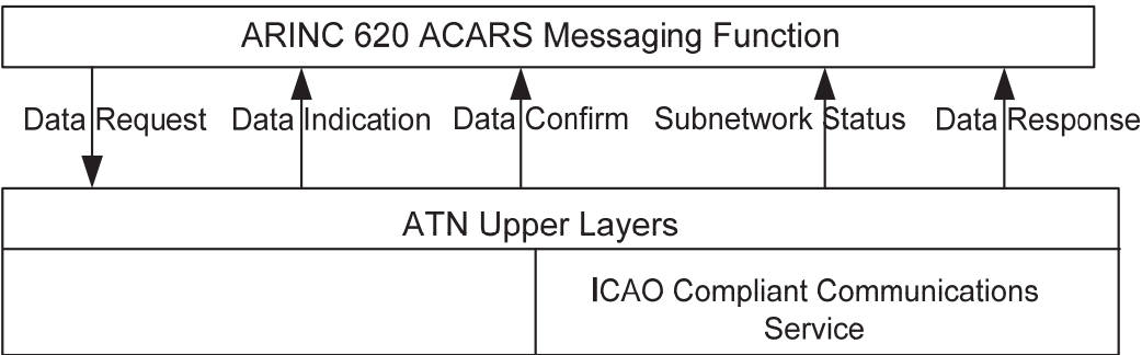
Figure 3.5-1 – Messaging Function Primitives
