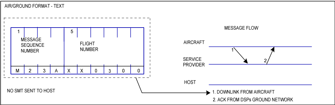
Figure 5.3.15-1 – Link Test
