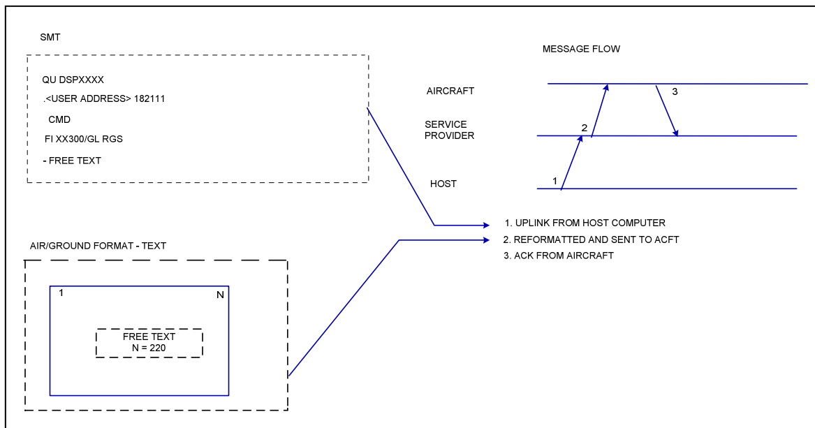
Figure 4.3.5-1 – Command/Response Uplink
