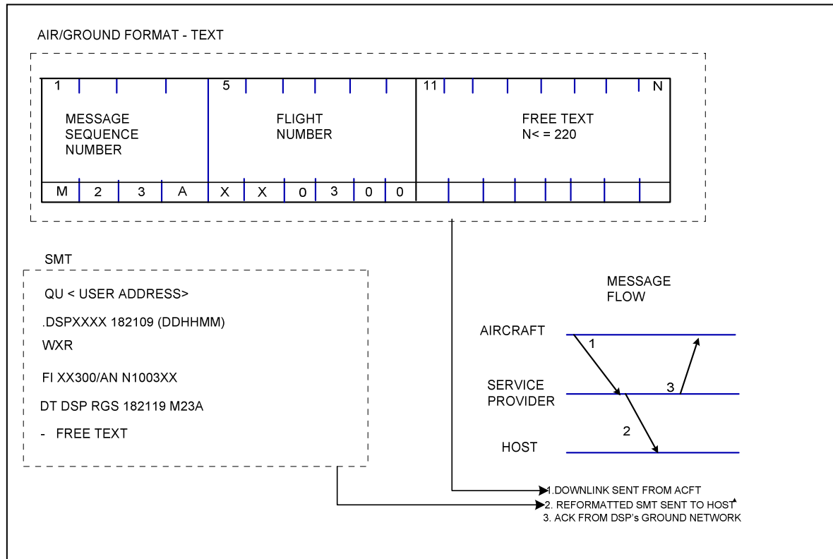
Figure 5.3.6-1 – Weather Request
