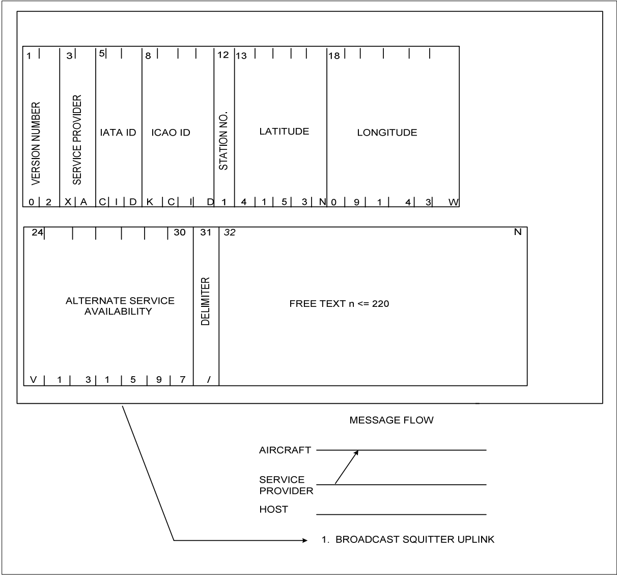
Figure 4.2.5-2 – Squitter Message, Version 2
