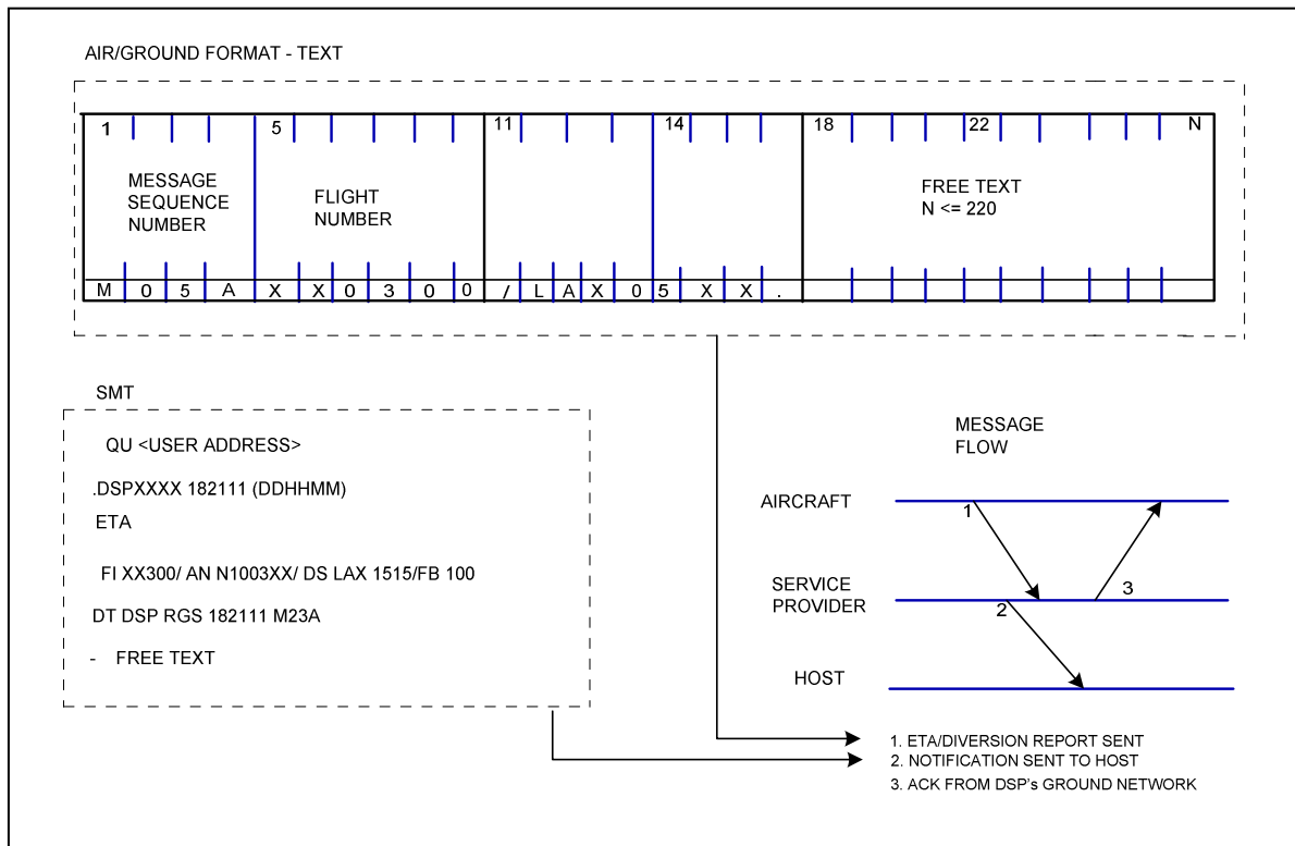
Figure 5.3.8 – ETA/Diversion Report
