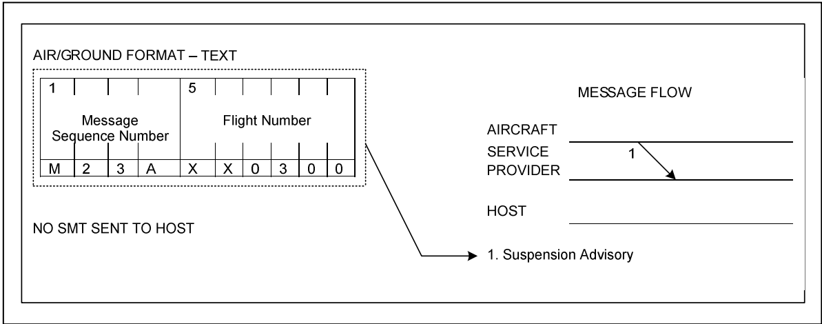
Figure 5.2.4-1 – Temporary Suspension
