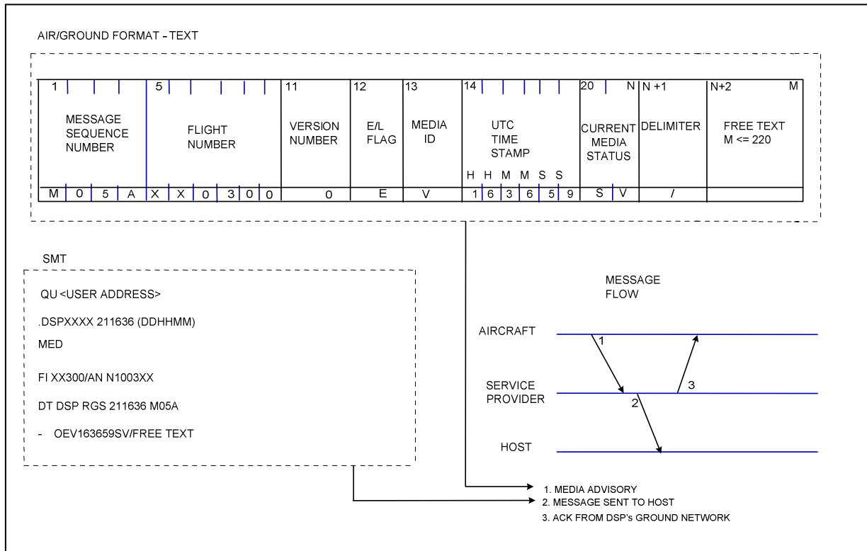
Figure 5.3.51-1 – Media Advisory
