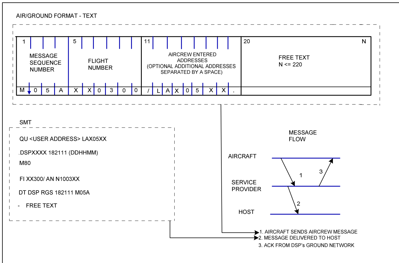
Figure 5.3.11-1 – Aircrew-Addressed Downlink
