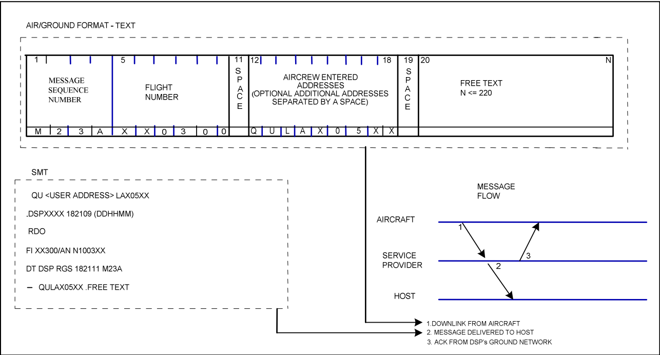
Figure 5.3.14-1 – Command/Response Downlink
