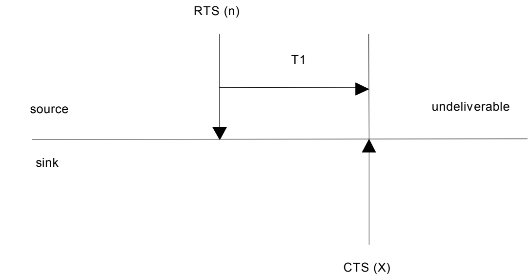
Figure 10-2 CTS Response
