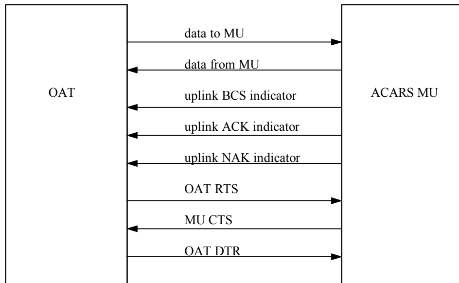
Figure 12.2-1 OAT/ACARS Interface
