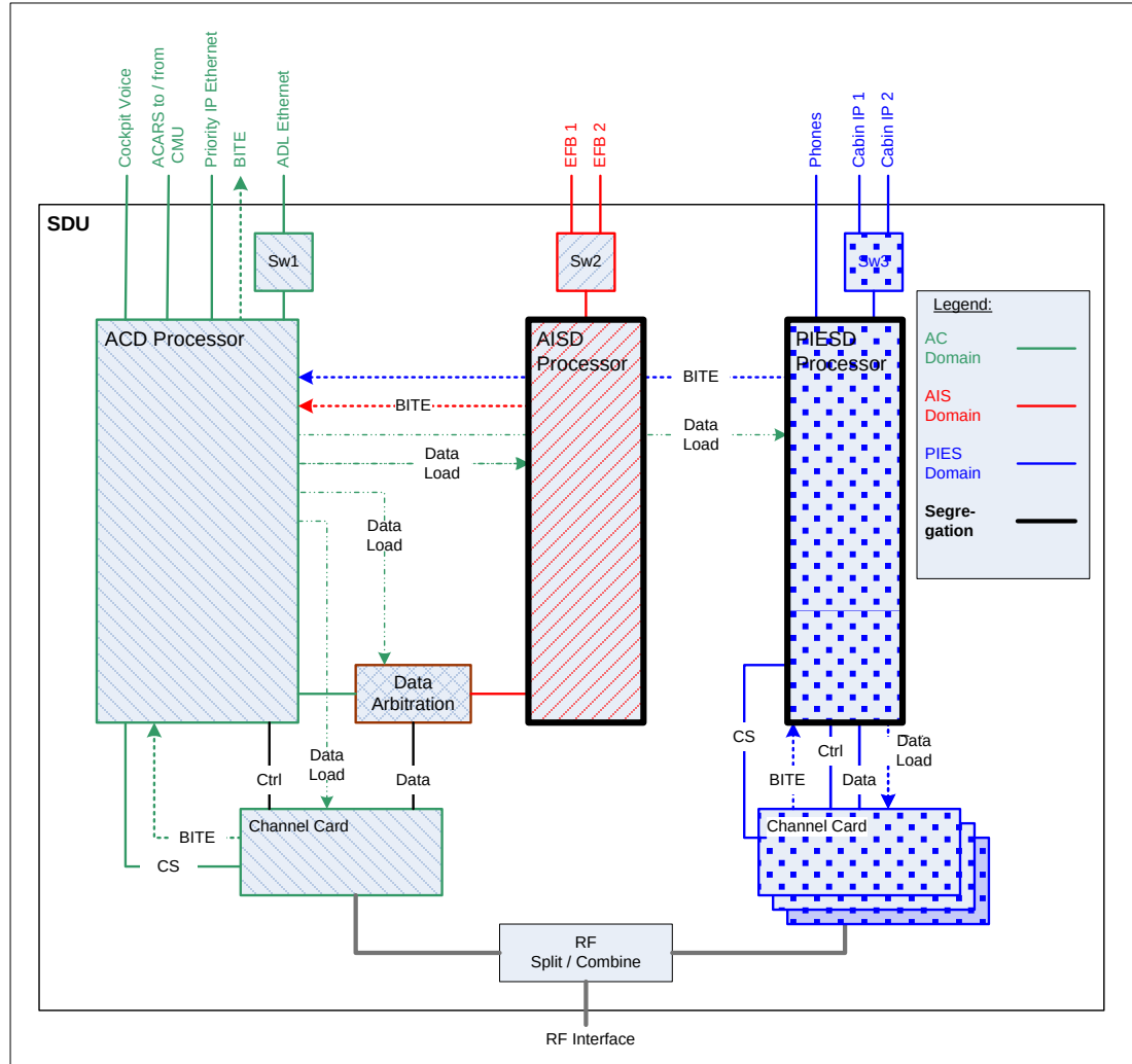
Figure 4 – Multi-Channel System Configuration 1
