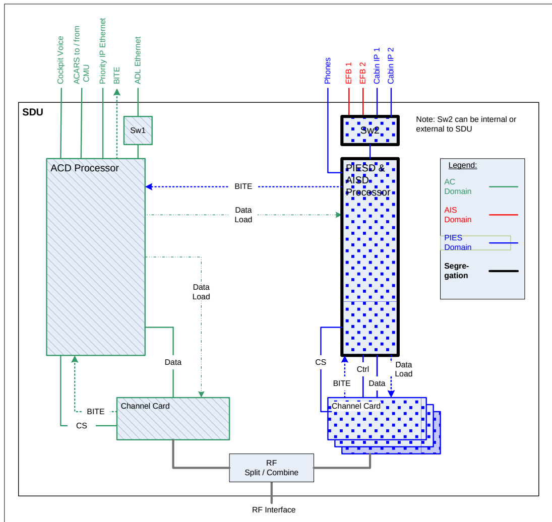
Figure 6 – Multi-Channel System Configuration 3
