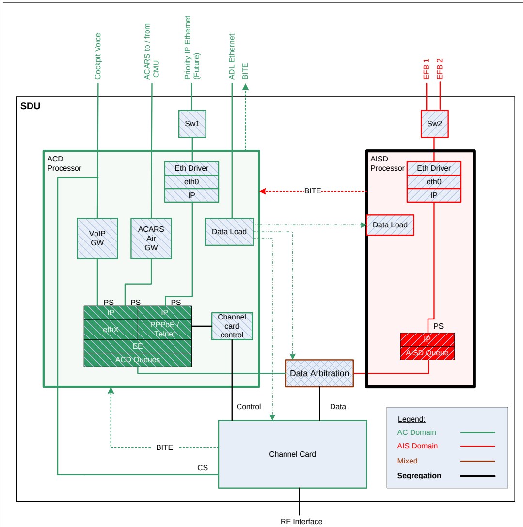
Figure 2 – Architecture for SB200-S Terminal
