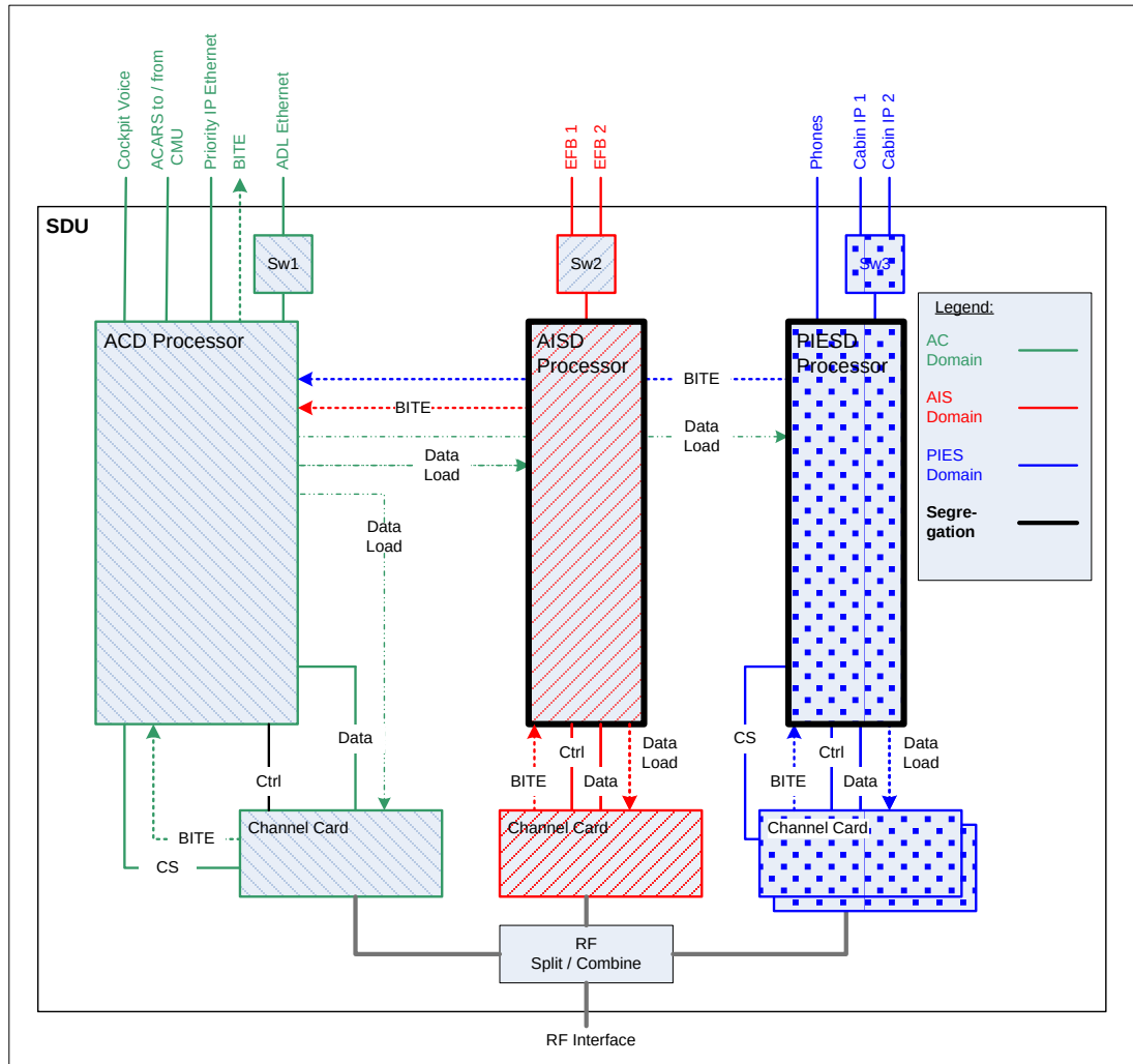
Figure 5 – Multi-Channel System Configuration 2
