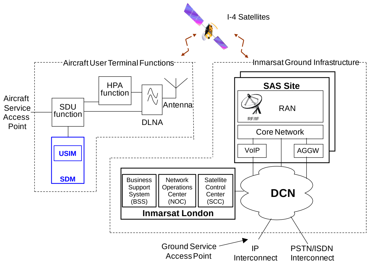
Figure 3-2 – Overall SwiftBroadband Architecture
