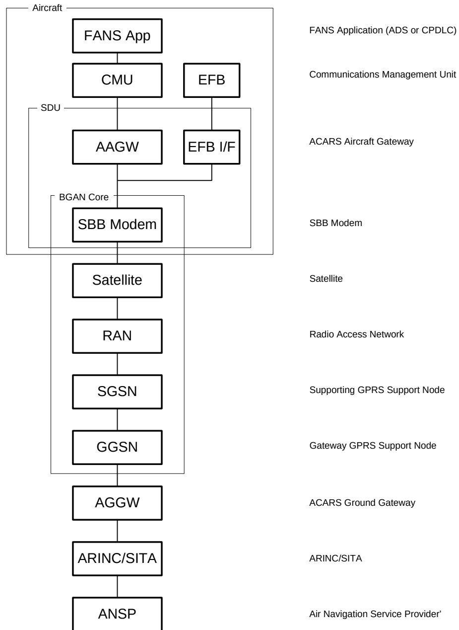
Figure 1 – End-to-End ACARS System Architecture
