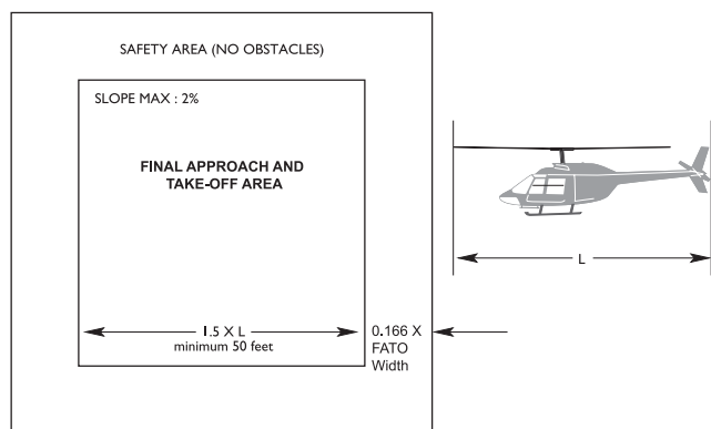
Figure 3.1—FATO/Safety Area
