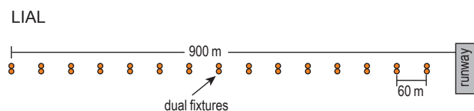
Figure 7.1—LIAL
