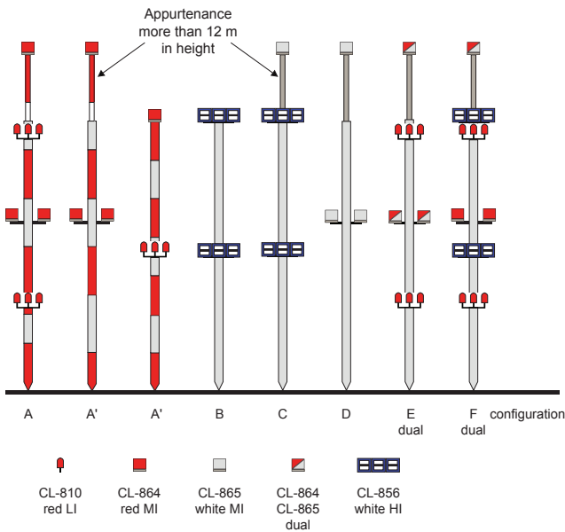
Figure 6.3—Configurations of Lighting on Skeletal Structures
