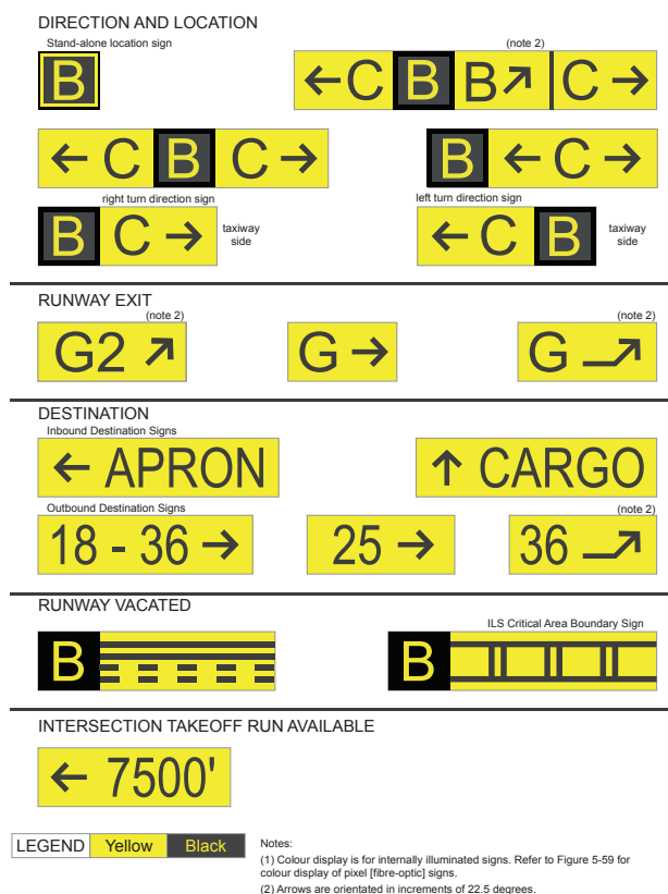
Figure 5.13—Information Signs
