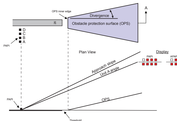
Figure 7.9—PAPI/APAPI OPS
