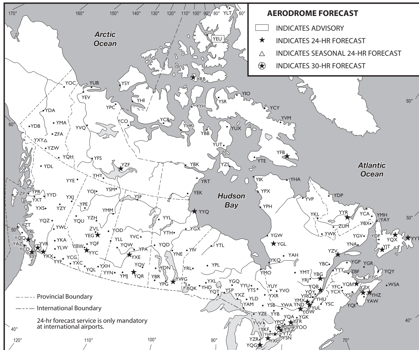
Figure 7.1—TAF Locations
