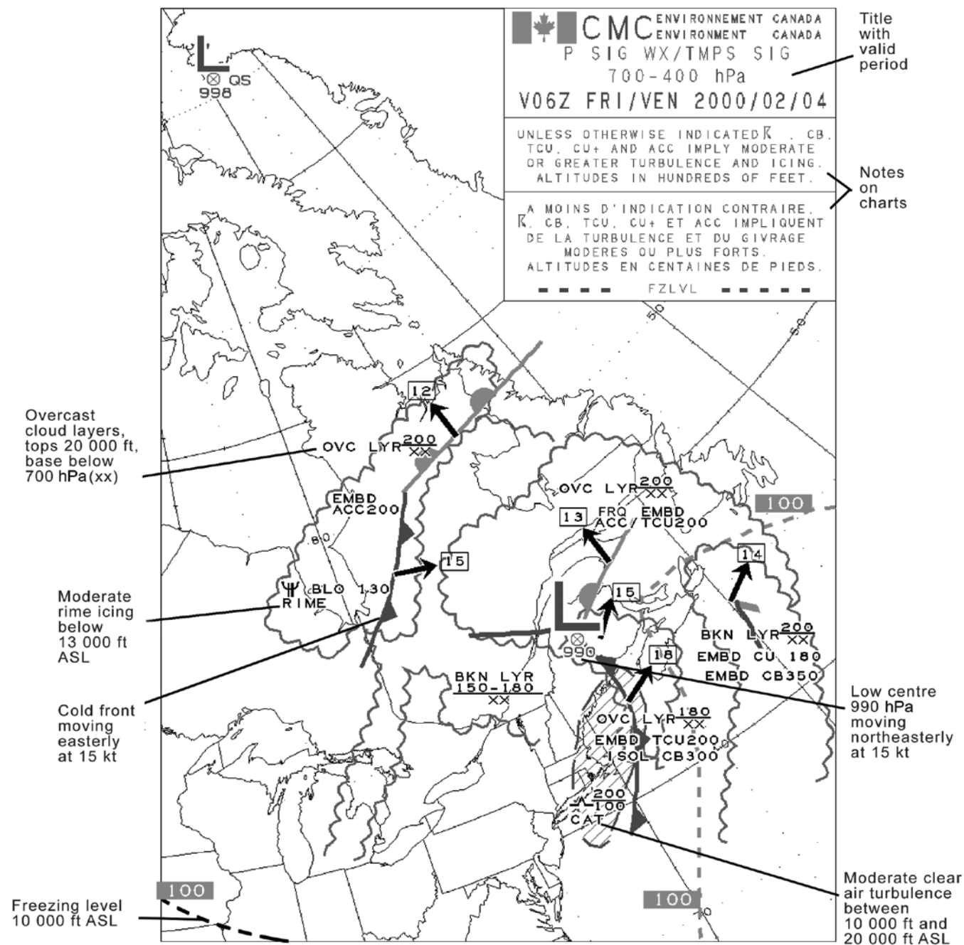
Figure 12.1(a)—Example of a Mid-Level Significant Weather Chart
