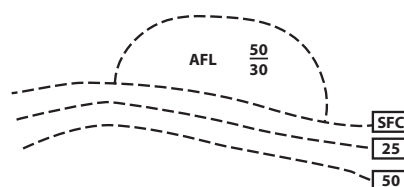
Figure 4.5(g)—Freezing Level
