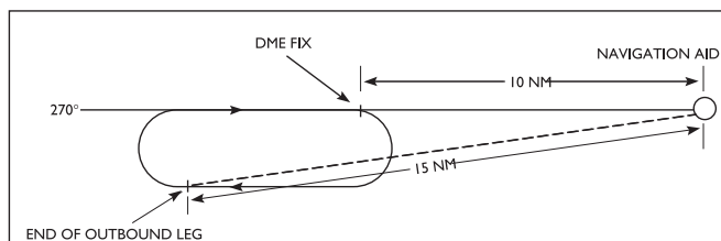
Figure 10.4—DME Hold
