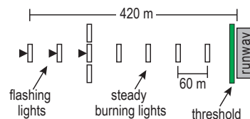
Figure 7.3—MALSF
