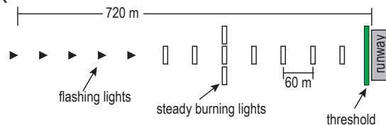
Figure 7.4—MALSR
