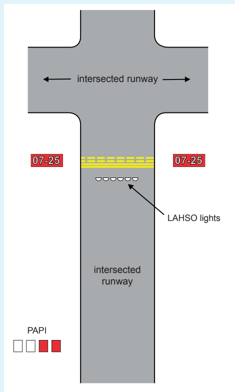
Figure 4.8—LAHSO Visual Aid Configuration
