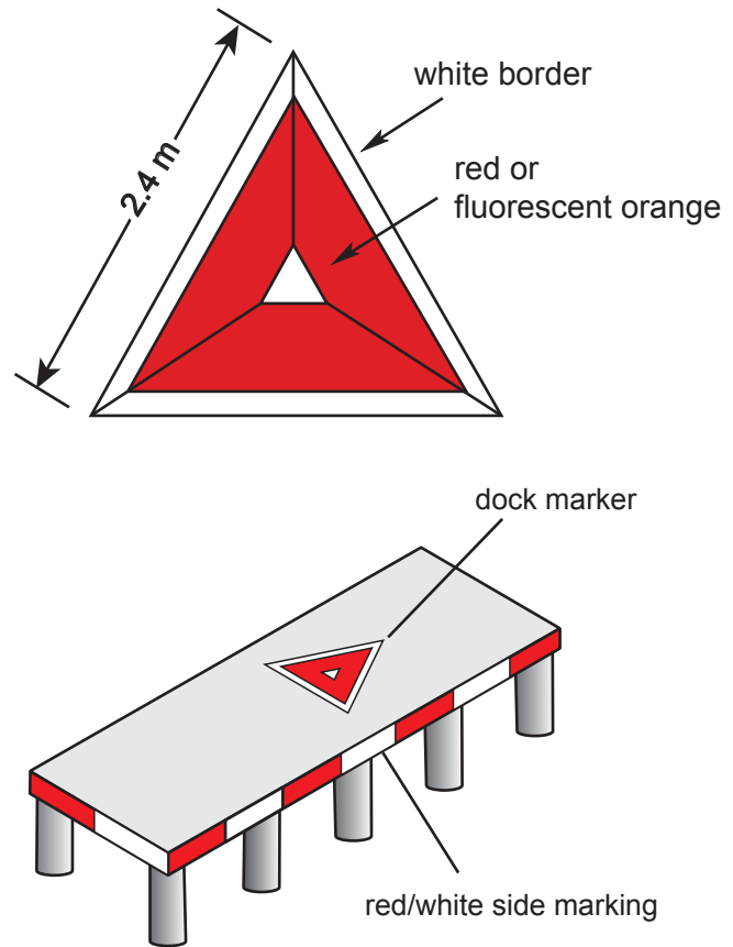
Figure 5.3—Seaplane Dock Markers
