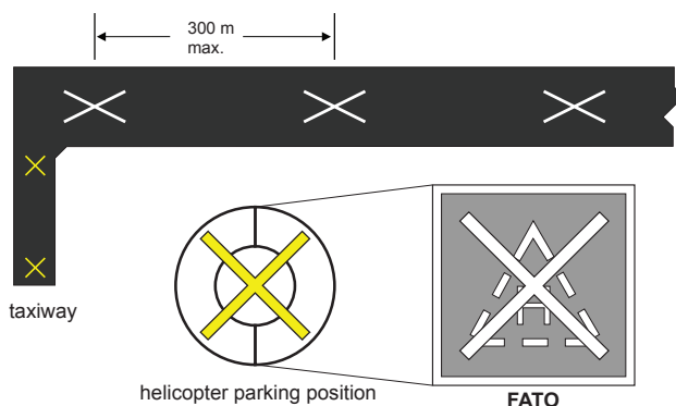
Figure 5.11—Closed Markings
