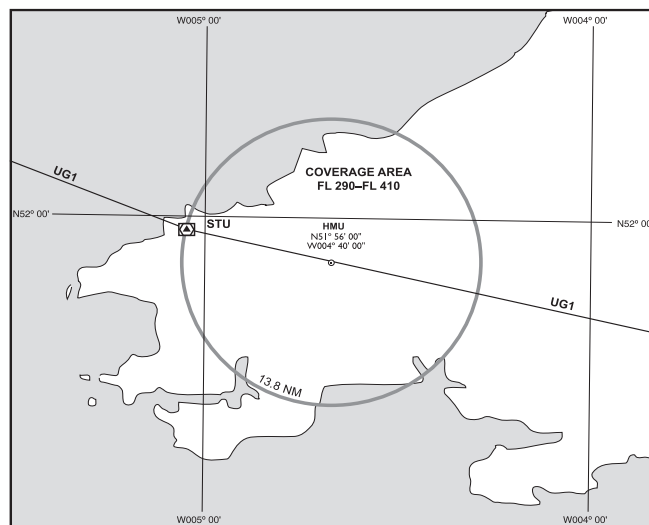
Figure 1.6—Strumble HMU
