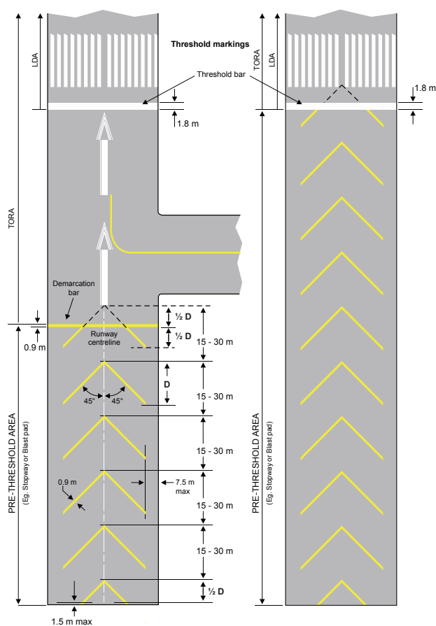
Figure 5.6—Stopway Markings
