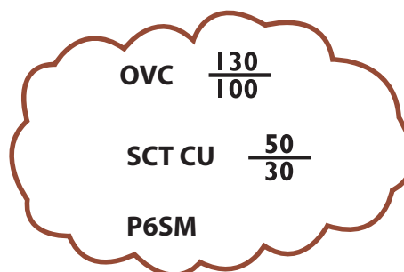
Figure 4.4(e)—Multiple Cloud Layers
