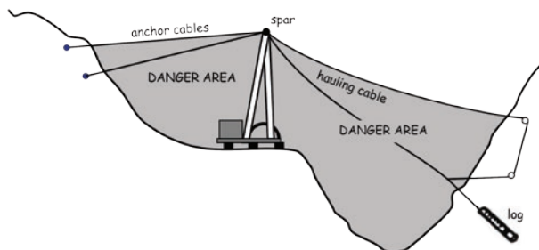
Figure 2.5—Highlead Spar
