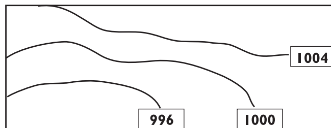
Figure 4.4(g)—Isobars
