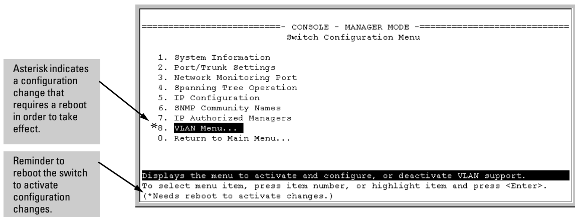
Figure 3-7. Indication of a Configuration Change Requiring a Reboot
