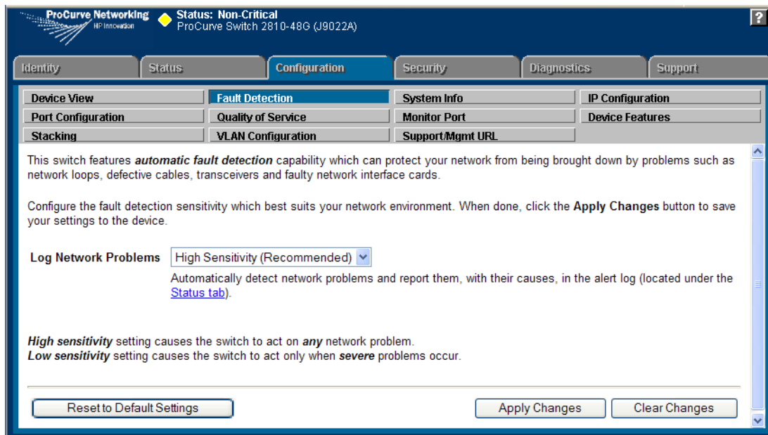
Figure 5-16. The Fault Detection Window
