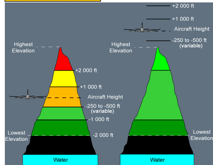
ND Terrain code color
