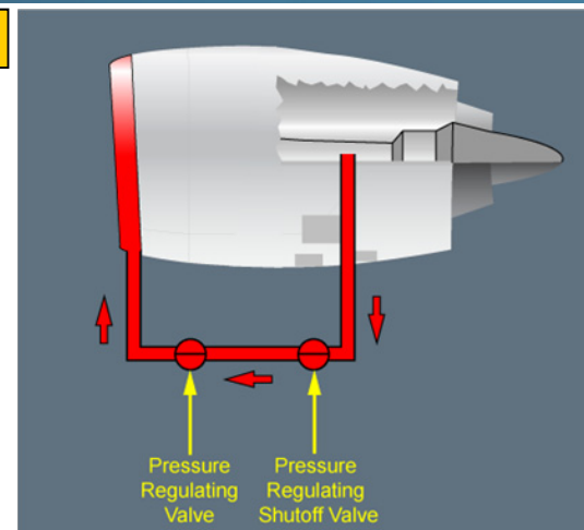
Engine Anti-Ice
