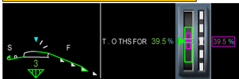
PFD: Slats/Flaps Spoilers and Pitch Trim Display
