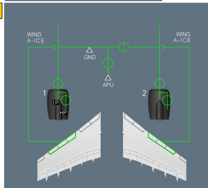
Wing Anti-Ice
